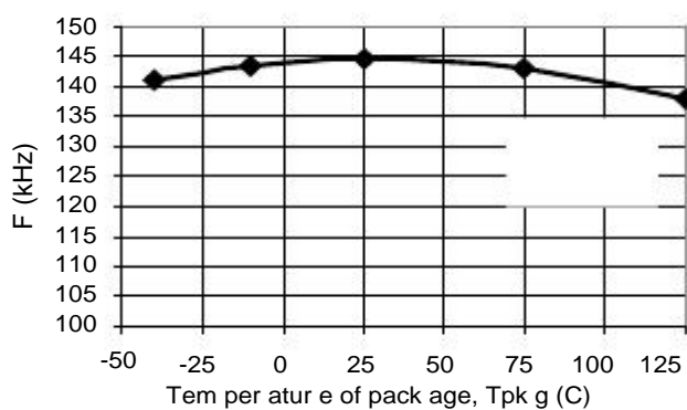
Frequency F vs Tpk g (TO-220)
