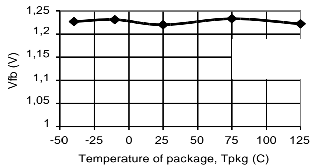
V_{fb} vs Tpk g (TO-220)
