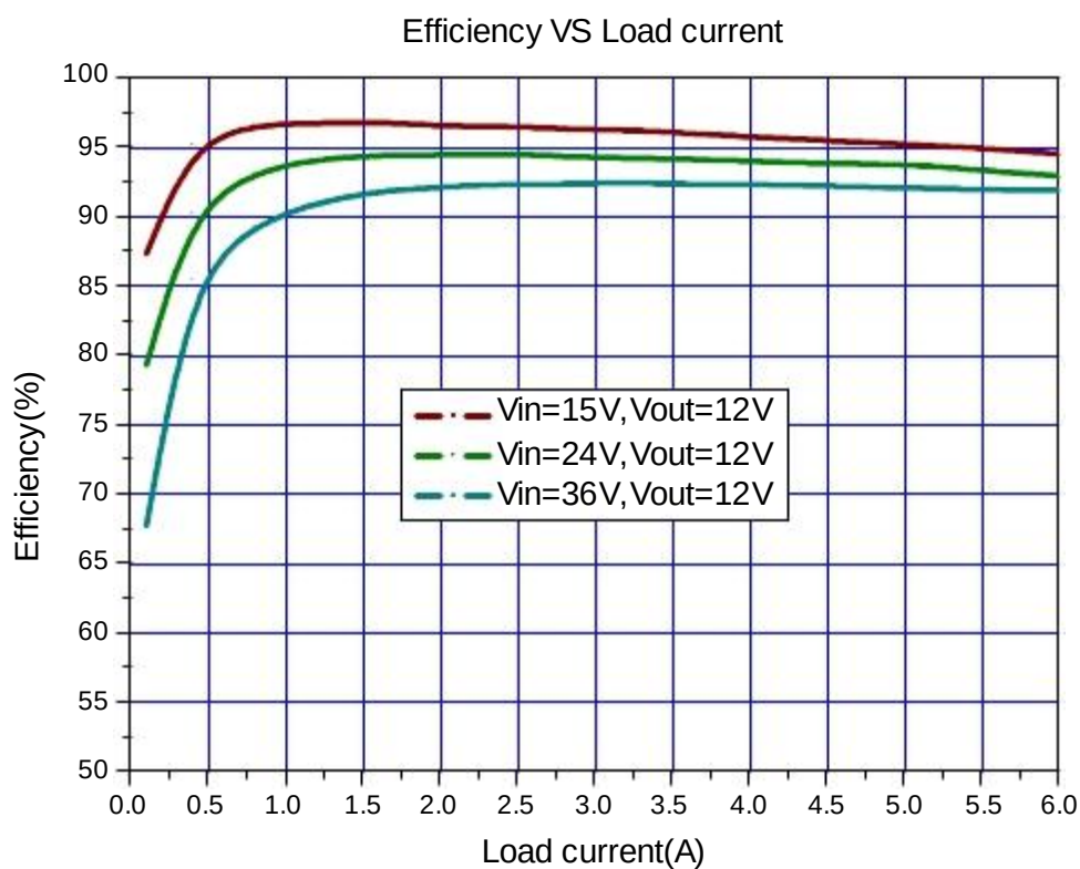
Figure8. JTM3105B System Efficiency Curve
