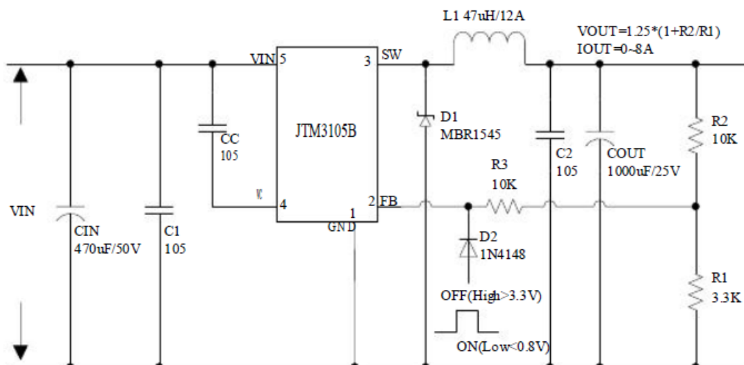
Figure7. JTM3105B System Parameters Test Circuit (VIN=15V~40V, VOUT=12V/6A)
