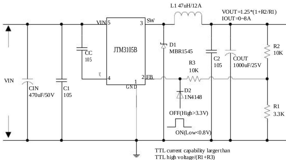
Figure9. JTM3105B Typical Application Circuit
