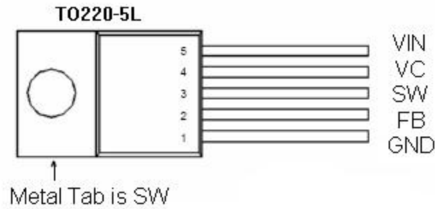
Figure2. Pin Configuration of JTM3105B (Top View)
