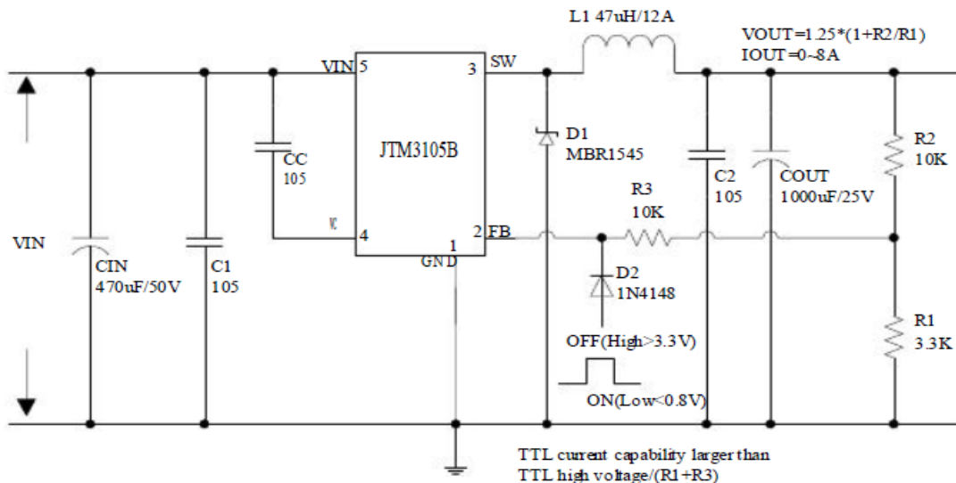
Figure5. JTM3105B System Parameters Test Circuit (VIN=8V~40V, VOUT=5V/8A)
