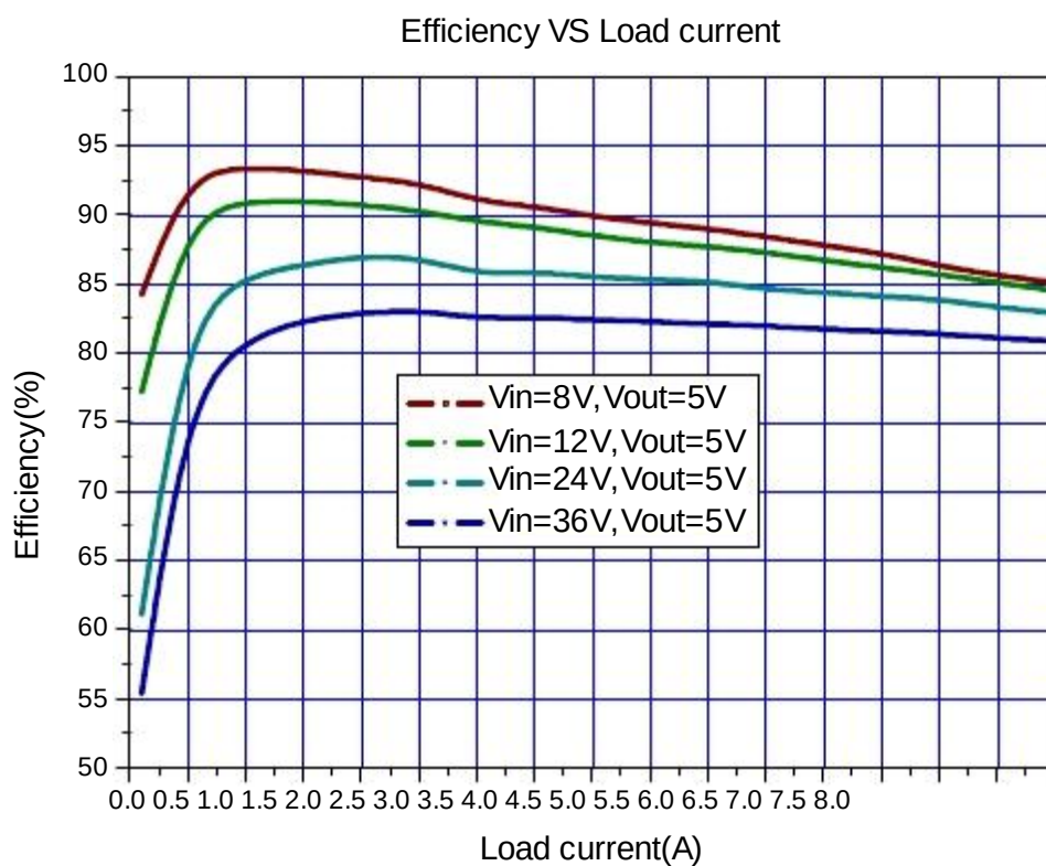
Figure6. JTM3105B System Efficiency Curve
