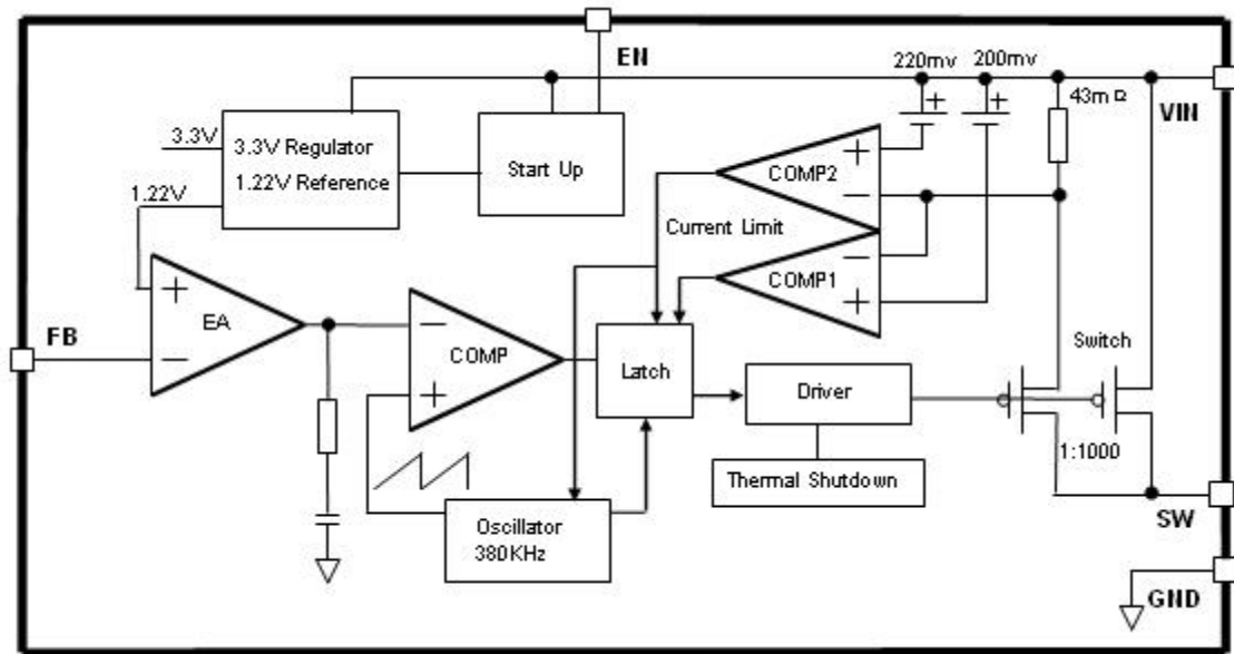
Figure3. Function Block Diagram of JTM1583
