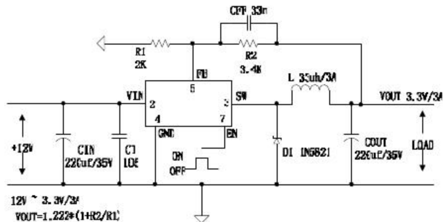
Figure7. JTM1583 System Parameters Test Circuit (12V ~ 3.3V/3A)
