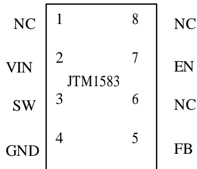
Figure2. Pin Configuration of JTM1583 (Top View)
