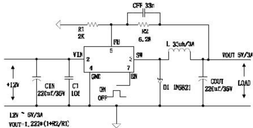
Figure6. JTM1583 System Parameters Test Circuit (12V ~ 5V/3A)
