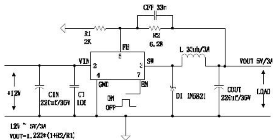
Figure4. JTM1583 Typical Application Circuit 12V-5V/3A
