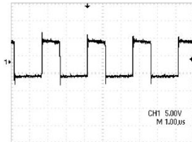
SW ( V_{IN}=9V , V_{OUT}=3.3V , I_{LOAD}=1A )
