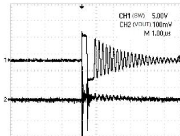
SW ( V_{IN}=9V , V_{OUT}=3.3V , I_{LOAD}=1A )
