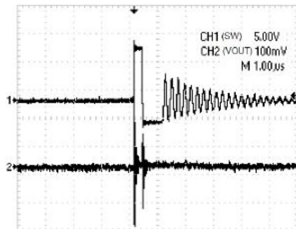
Start-up from Shutdown ( V_{IN}=12V )
