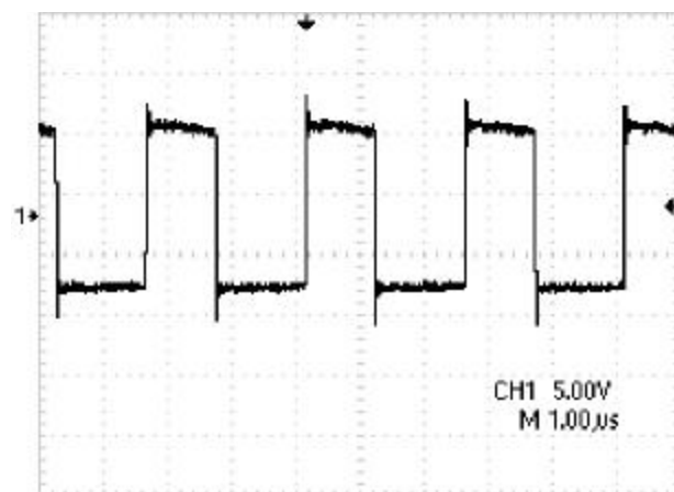
SW ( V_{IN}=12V , V_{OUT}=3.3V , I_{LOAD}=1A )
