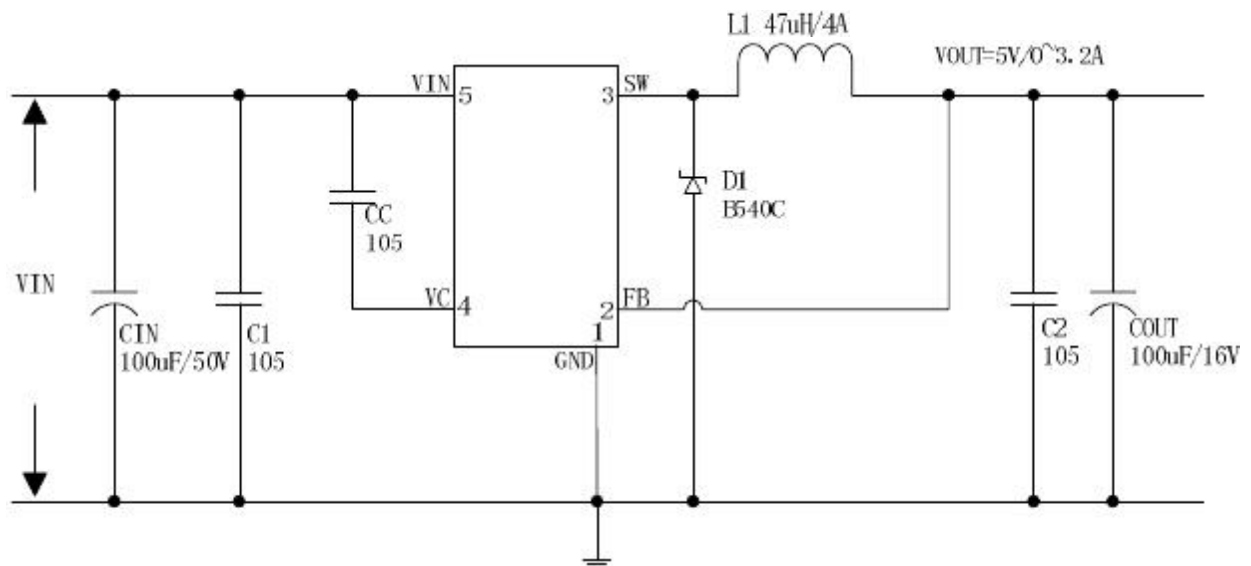
Figure4. JTM3513 Typical Application Circuit (VIN=8V~40V, VOUT=5V/3.2A)
