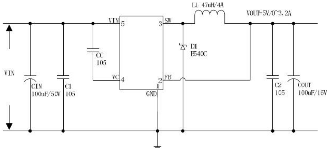
Figure5. JTM3513 System Parameters Test Circuit (VIN=8V~40V, VOUT=5V/3.2A)
