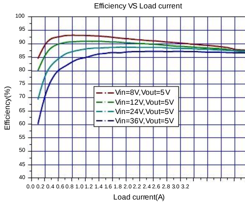
Figure7. JTM3513 System Efficiency Curve
