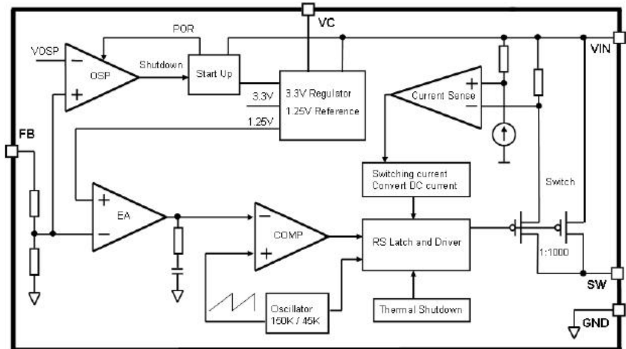
Figure3. Function Block Diagram of JTM3513
