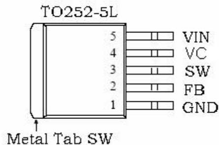
Figure2. Pin Configuration of JTM3513 (Top View)
