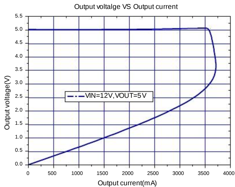
Figure6. JTM3513 System Output Constant Current Curve
