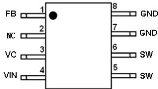
Figure2. Pin Configuration of JTM3501 (Top View)
