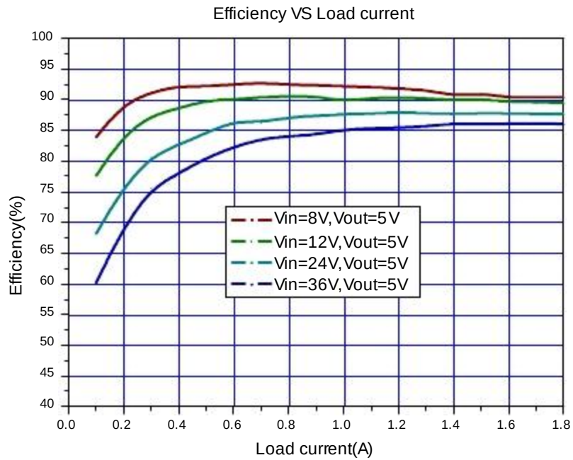
Figure7. JTM3501 System Efficiency Curve
