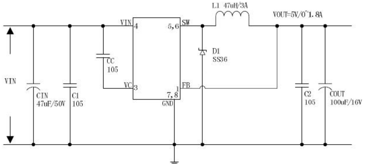
Figure5. JTM3501System Parameters Test Circuit (VIN=8V~45V, VOUT=5V/1.8A)
