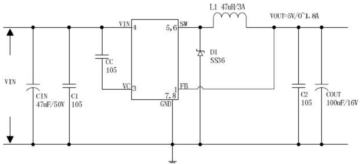
Figure4. JTM3501 Typical Application Circuit (VIN=8V~45V, VOUT=5V/1.8A)
