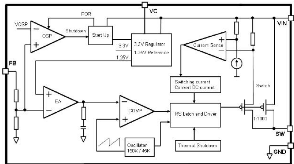
Figure3. Function Block Diagram of JTM3501
