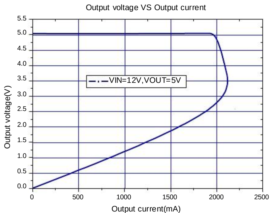
Figure6. JTM3501 System Output Constant Current Curve
