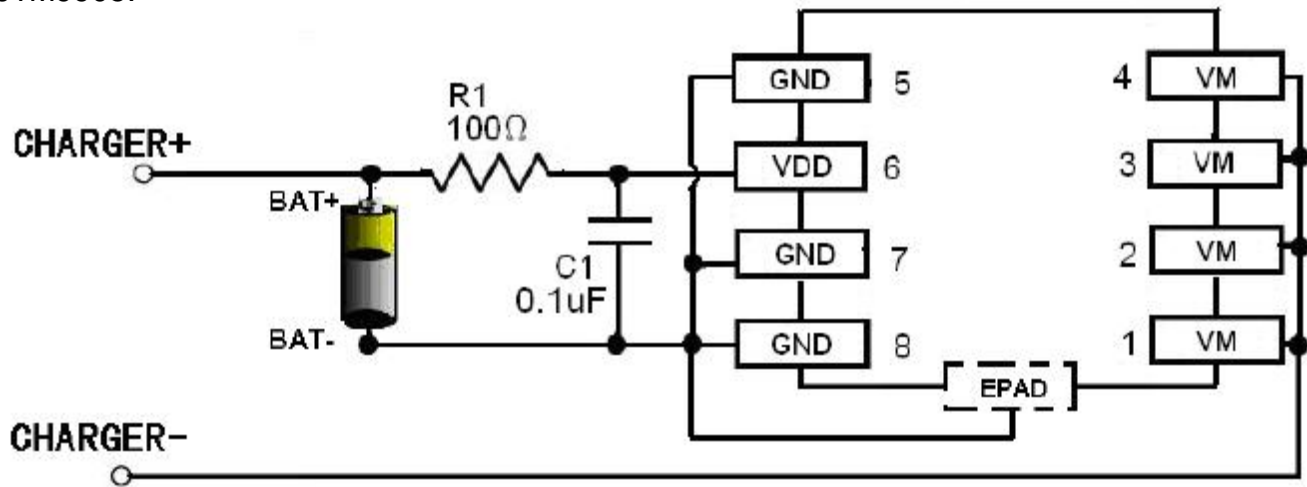
Fig 6 JTM9905 in a Typical Battery Protection Circuit
