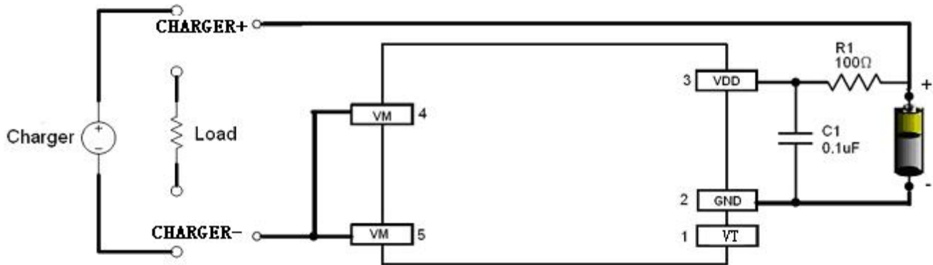
Fig 6 JTM5453A in a Typical Battery Protection Circuit
