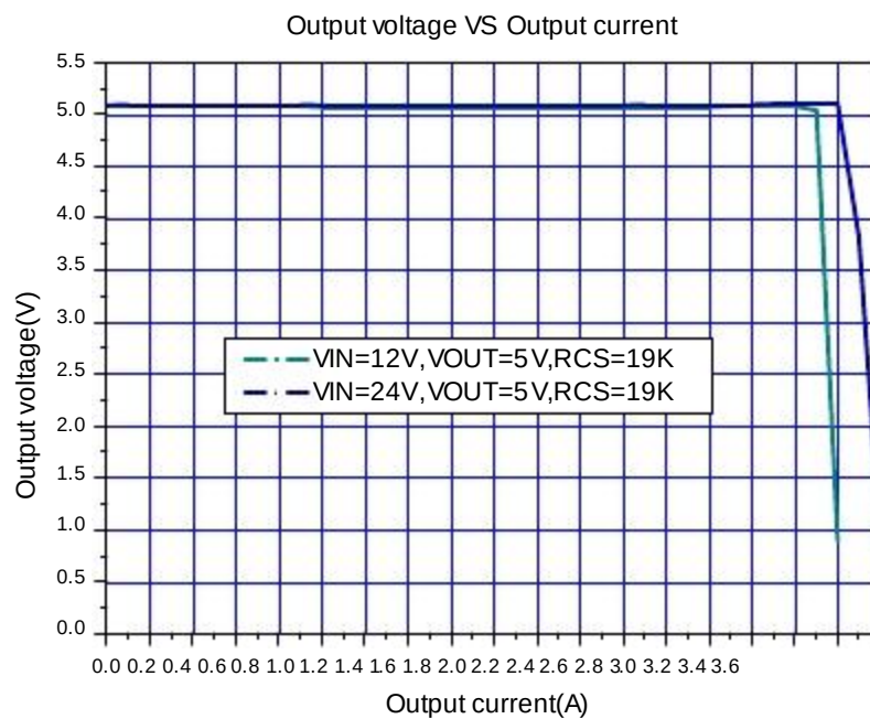
Figure6. JTM3108 System Output Constant Current Curve
