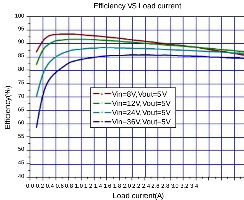
Figure7. JTM3108 System Efficiency Curve
