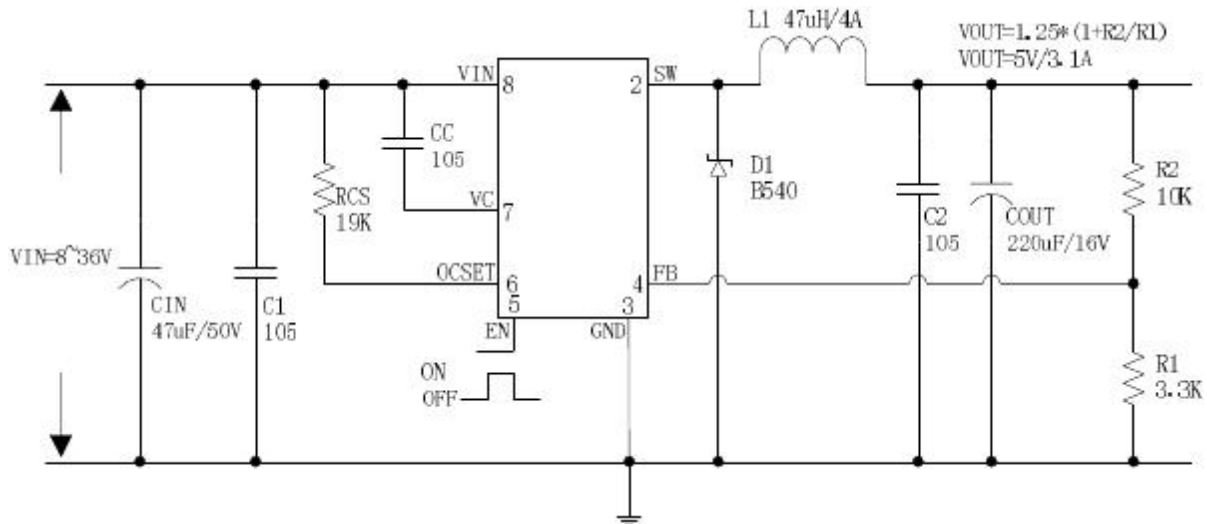
Figure5. JTM3108 System Parameters Test Circuit (VIN=8V~36V, VOUT=5V/3.1A)
