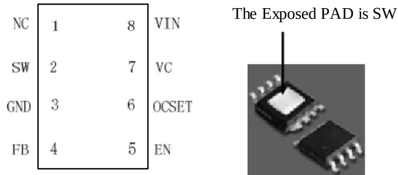
Figure2. Pin Configuration of JTM3108 (Top View)
