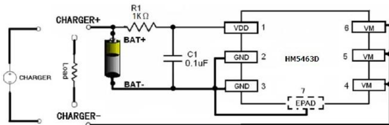
Fig.39 JTM5463D Typical Battery Protection Circuit
