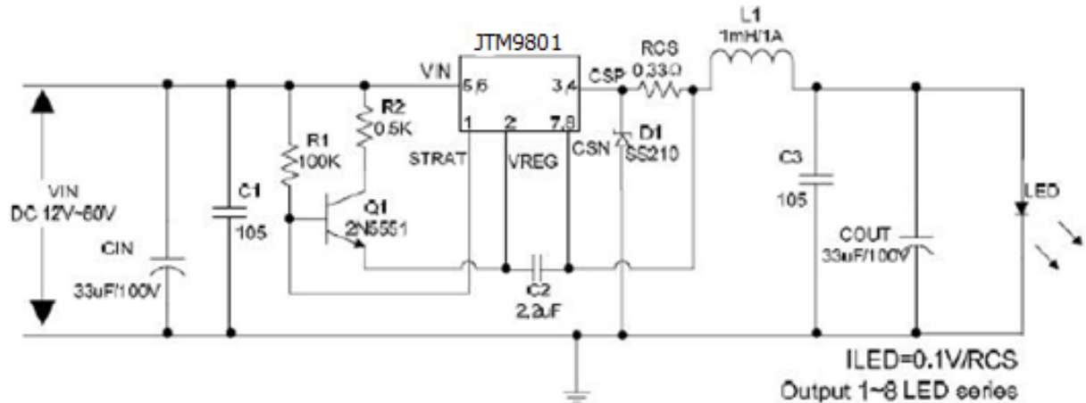
Figure5. JTM9801 System Application at VIN=12V~80V Schematic
