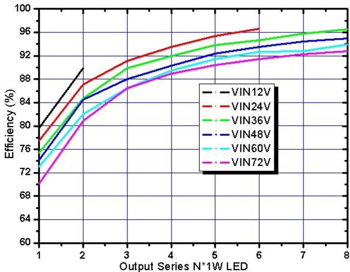
Figure6. JTM9801 System Application at VIN=12V~80V Efficiency Curve
