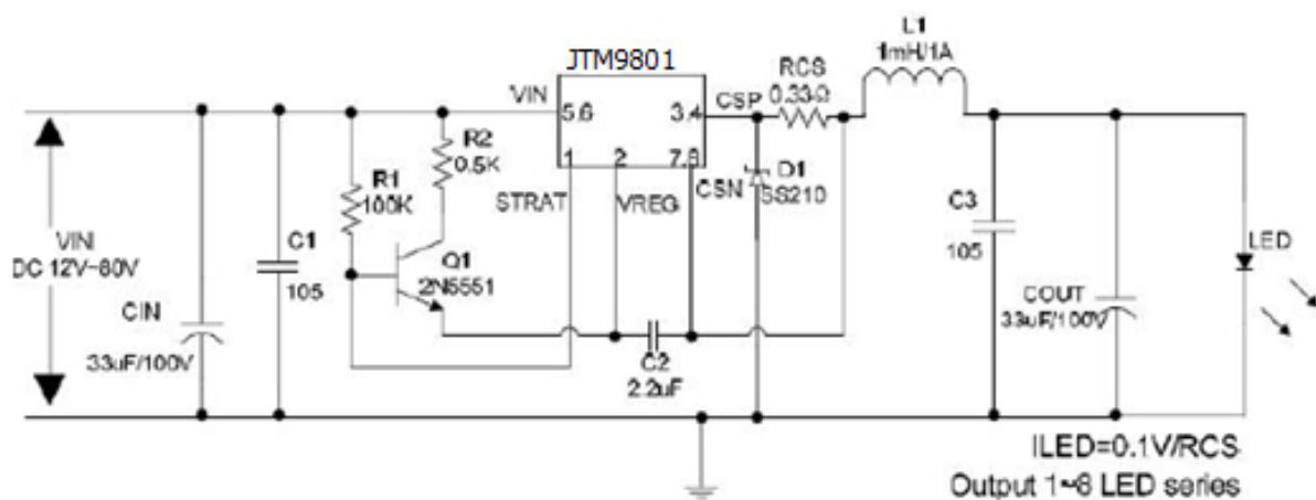
Figure4. JTM9801 Typical Application
