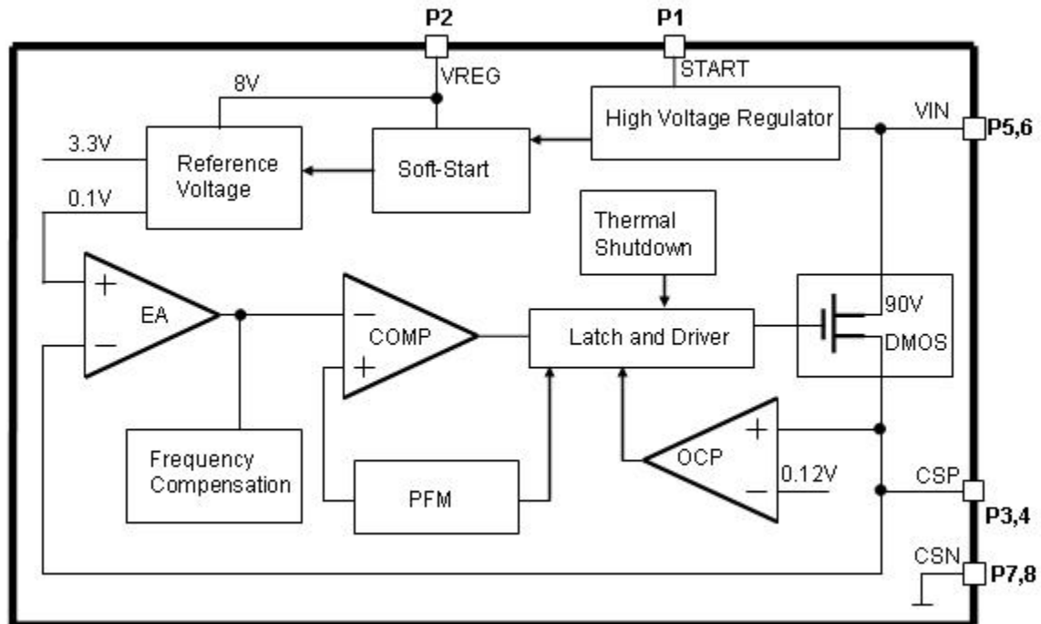
Figure3. Function Block Diagram of JTM9801
