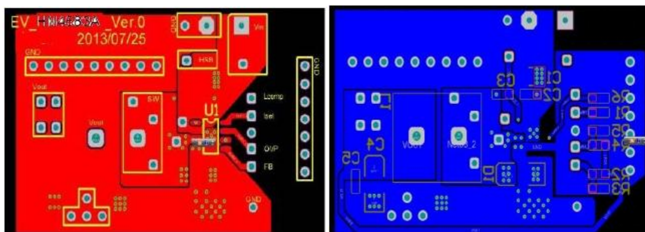
Figure 6: PCB Layout
