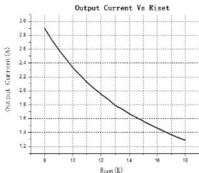
Curve for Programming Output CC Current
