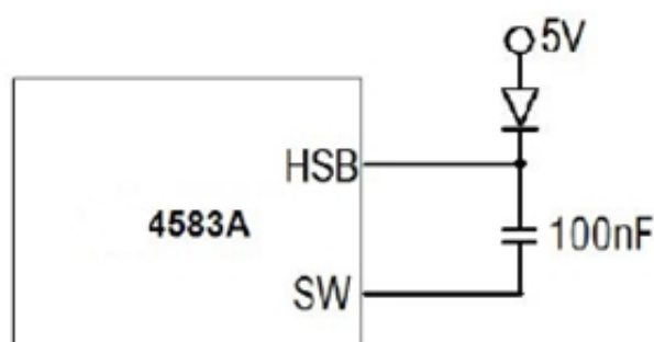
Figure 4: External High Voltage Bias Diode
