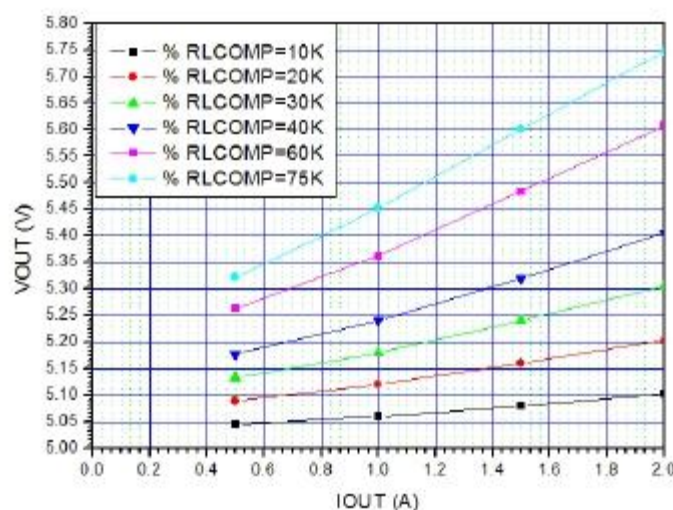
Figure 5: Cable Compensation
