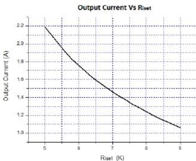
Curve for Programming Output CC Current
