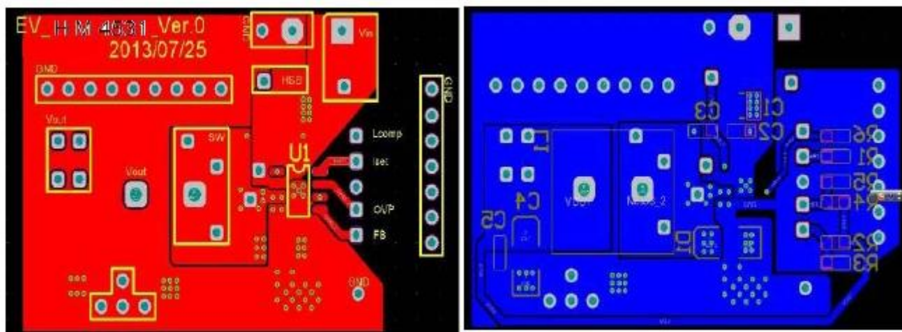
Figure 6: PCB Layout
