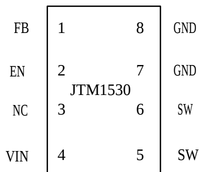
Figure2. Pin Configuration of JTM1530 (Top View)
