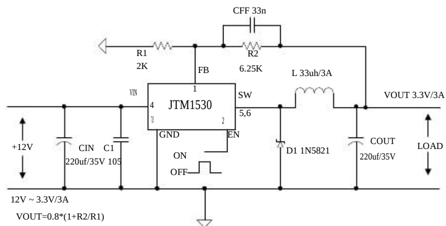
Figure7. JTM1530 System Parameters Test Circuit (12V ~ 3.3V/3A)
