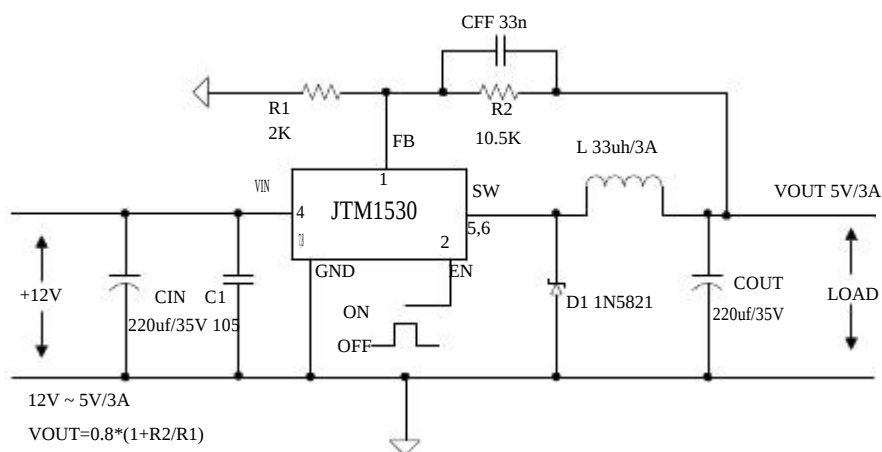
Figure6. JTM1530 System Parameters Test Circuit (12V ~ 5V/3A)
