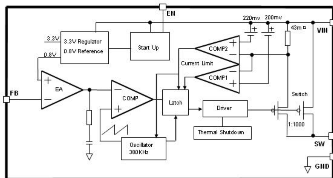
Figure3. Function Block Diagram of JTM1530
