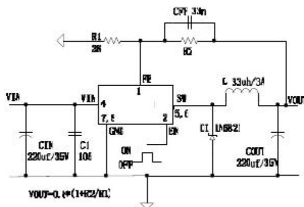
Figure4. JTM1530 Typical Application Circuit
