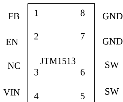
Figure2. Pin Configuration of JTM1513 (Top View)
