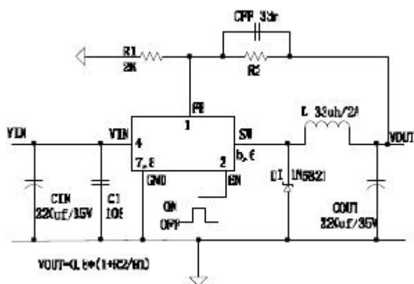
Figure4. JTM1513 Typical Application Circuit
