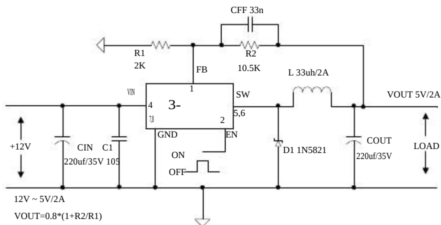
Figure6. JTM1513 System Parameters Test Circuit (12V ~ 5V/2A)
