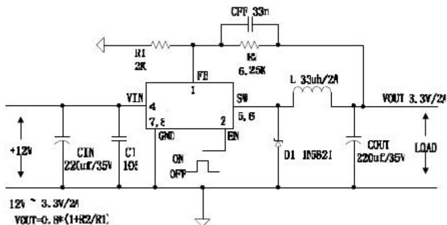
Figure7. JTM1513 System Parameters Test Circuit (12V ~ 3.3V/2A)
