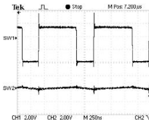
Switch Pins in Buck Mode ( V_{IN}=5V , V_{OUT}=3.3V , I_{LOAD}=250mA )
