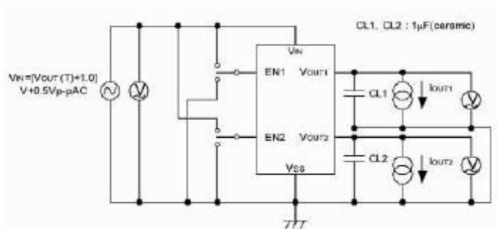
Circuit ⑤
