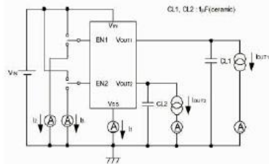
Circuit ②
