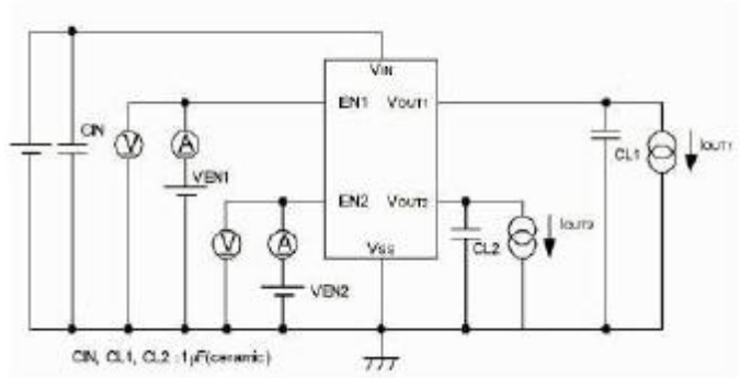
Circuit ④
