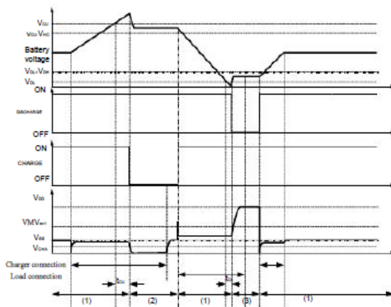
Figure5-1 Overcharge and Overdischarge Voltage Detection
