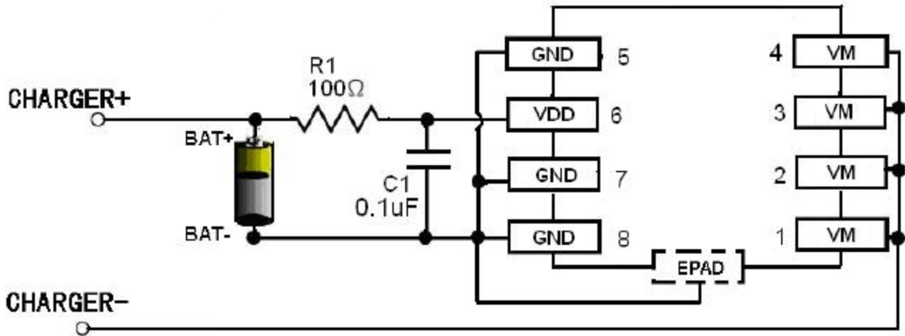
Fig 6 JTM9903 in a Typical Battery Protection Circuit
