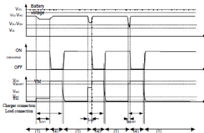
Figure5-2 Overdischarge Current Detection
