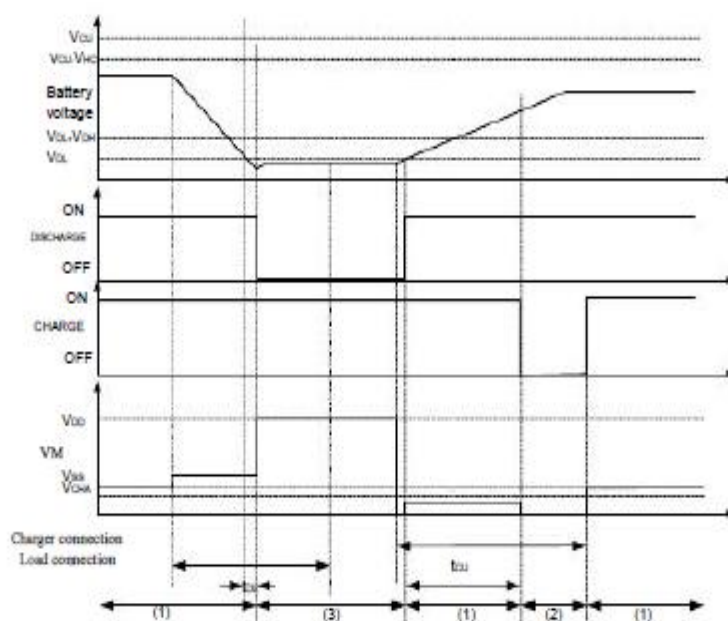
Figure5-4 Abnormal Charger Detection
