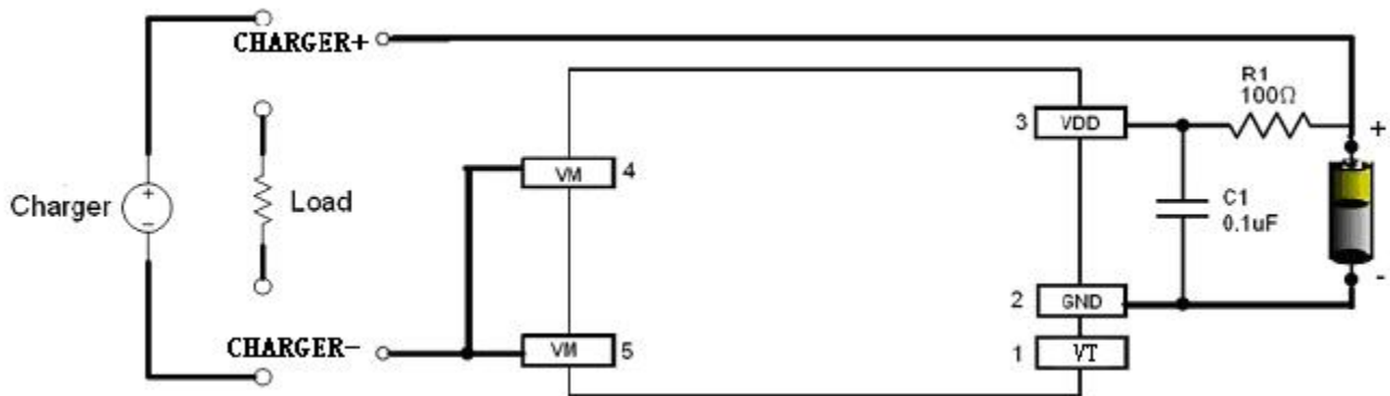
Fig 6 JTM5451 in a Typical Battery Protection Circuit
