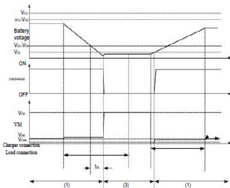
Figure5-3 Charger Detection
