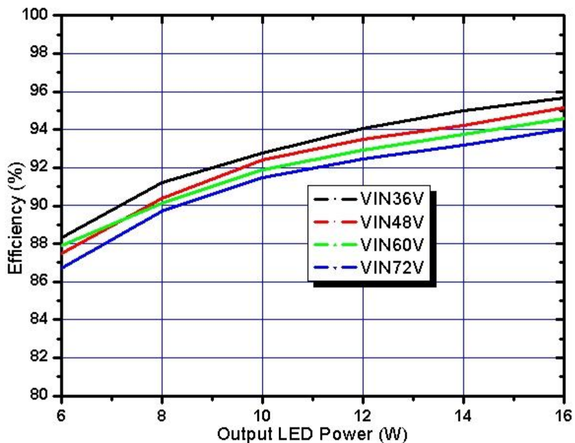
Figure8. JTM9804 System efficiency curve
