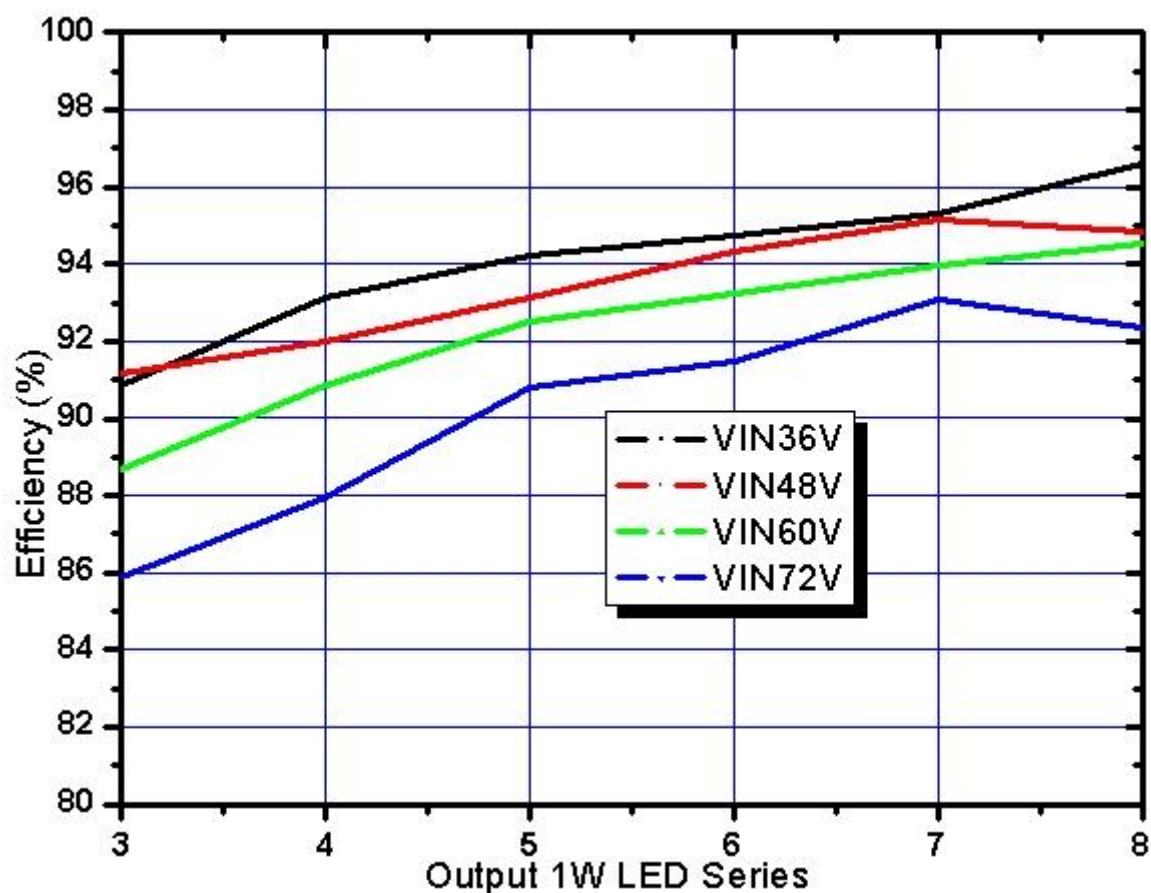
Figure6. JTM9804 System efficiency curve
