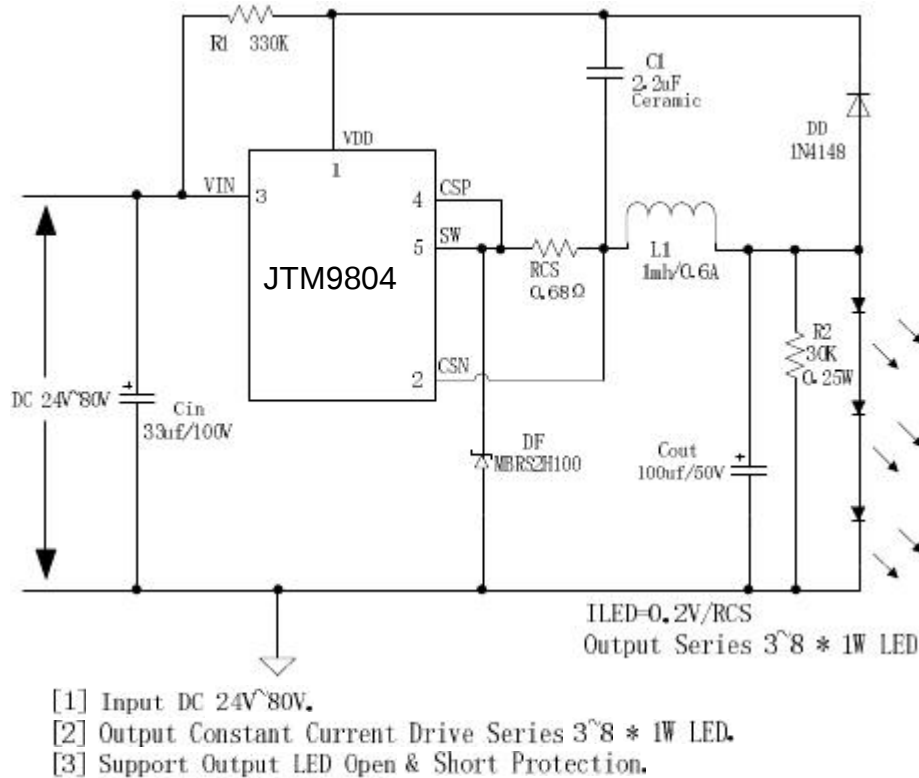
Figure4. JTM9804 Typical Application (3W~8W LED lamp)
