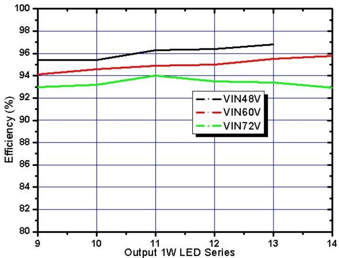
Figure10. JTM9804 System efficiency curve
