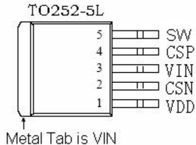
Figure2. Pin Configuration of JTM9804 (Top View)
