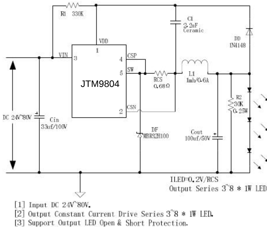
Figure5. JTM9804 System Application (3W ~ 8W)
