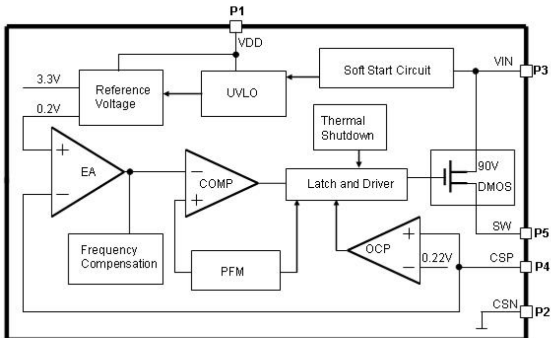
Figure3. Function Block Diagram of JTM9804
