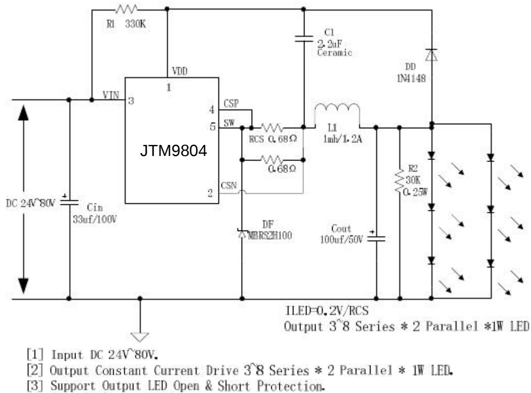
Figure7. JTM9804 System Application (6W ~ 16W)
