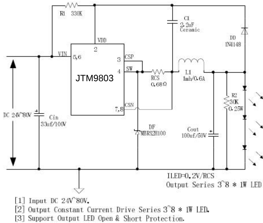
Figure5. JTM9803 System Application (3W ~ 8W)
