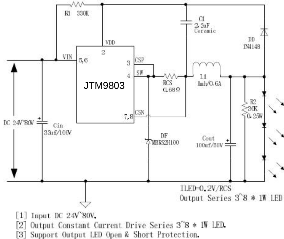
Figure4. JTM9803 Typical Application (3W~8W LED lamp)
