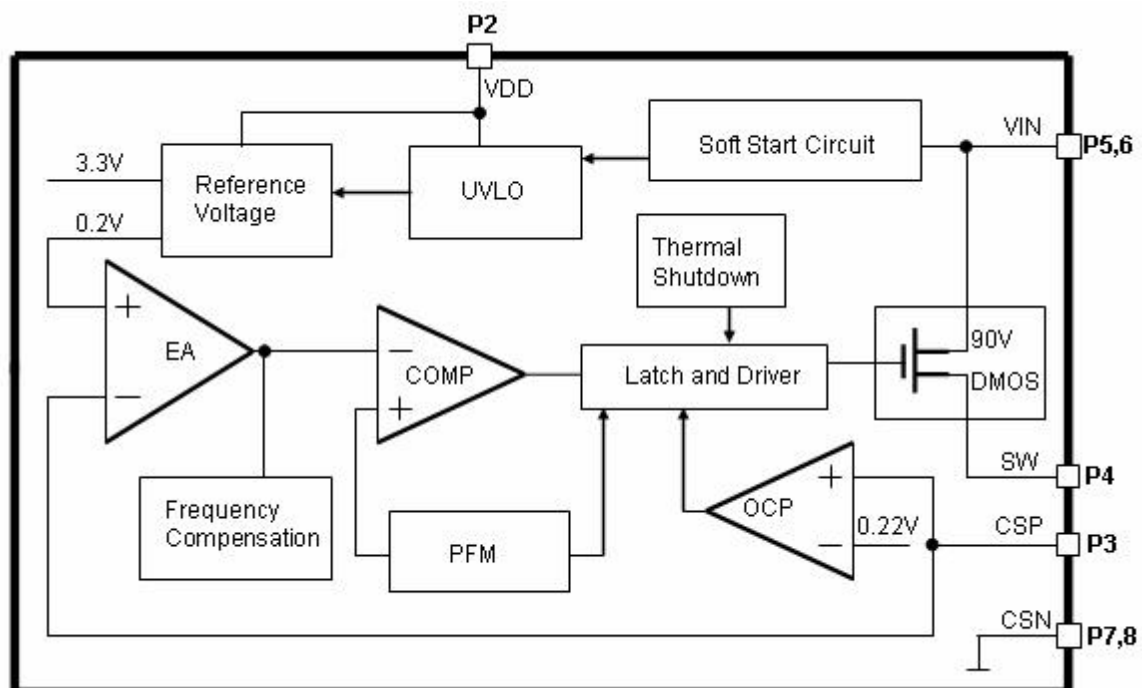
Figure3. Function Block Diagram of JTM9803
