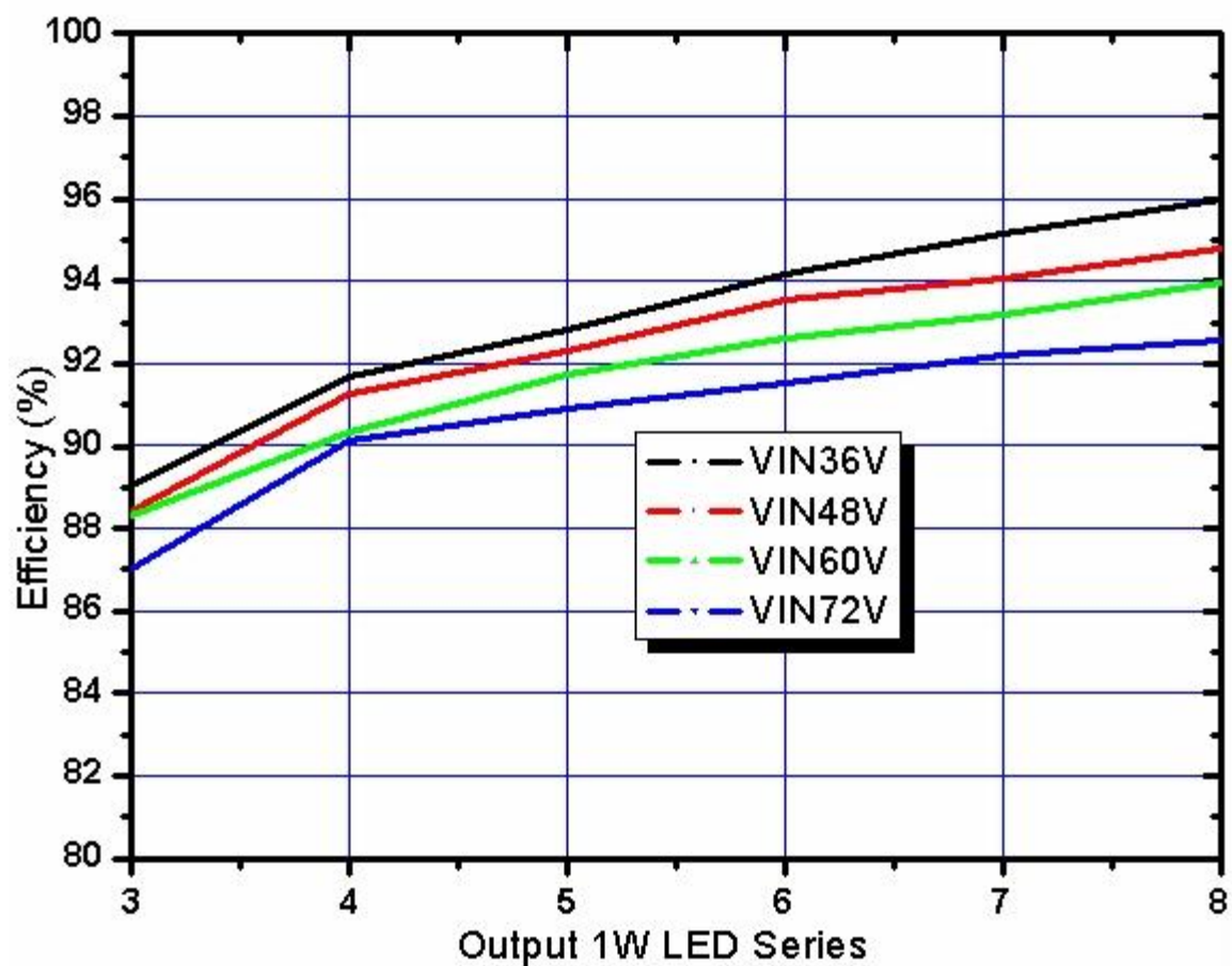
Figure6. JTM9803 System efficiency curve
