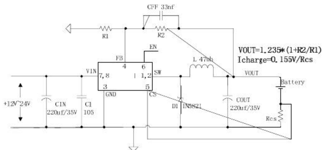
Figure4. JTM3101 Typical Application Circuit (Li Battery Charger)
