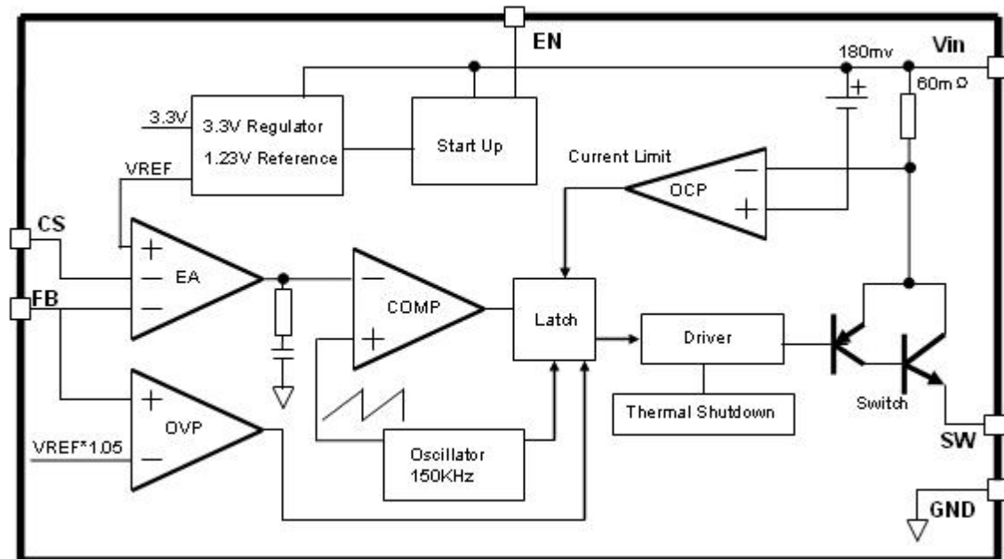
Figure3. Function Block Diagram of JTM3101
