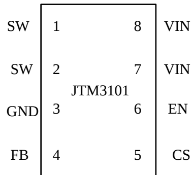
Figure2. Pin Configuration of JTM3101 (Top View)
