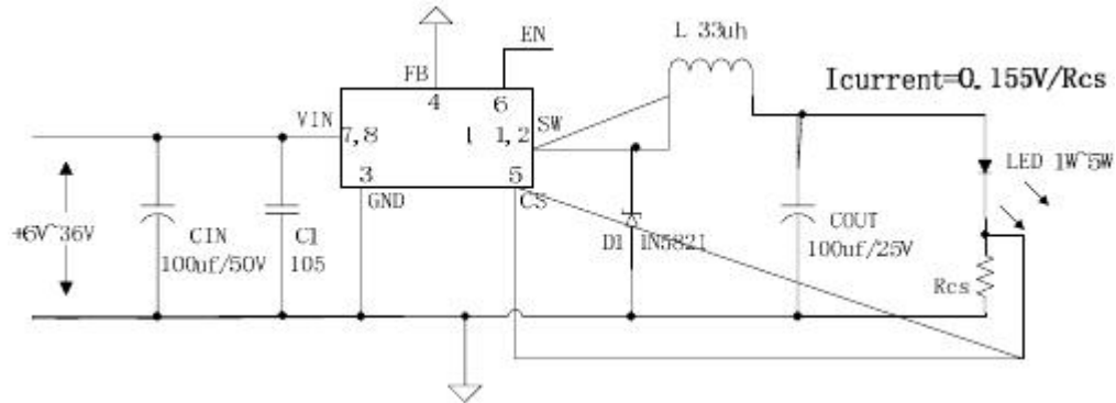
Figure5. JTM3101 Typical Application Circuit (LED Constant Current Driver)
