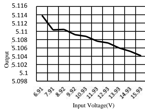
Line Regulation
