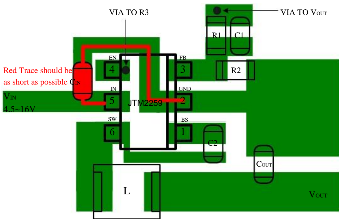
Figure 3. JTM2259 Suggested Layout
