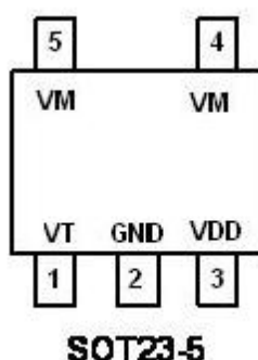
Figure 2. PIN Configuration
