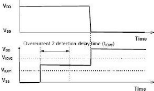
Figure 4. Overcurrent delay time
