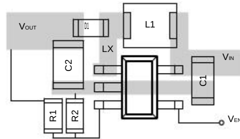
Optimized JTMA7137 Layout
