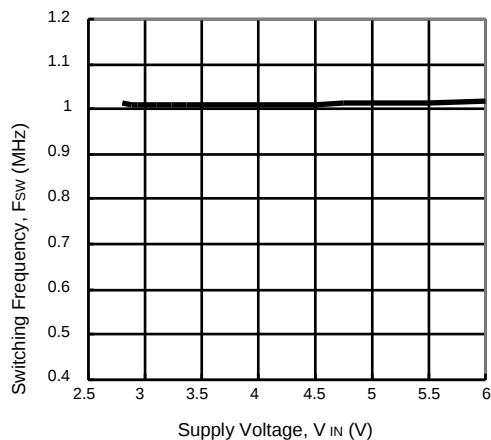
Switching Frequency vs. Supply Voltage
