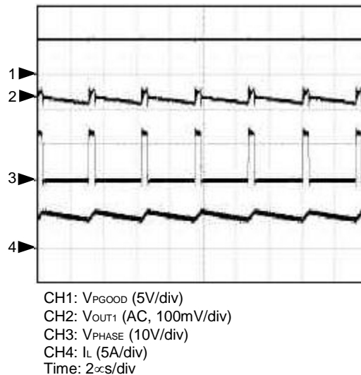
Operating at Heavy Load of 5A
