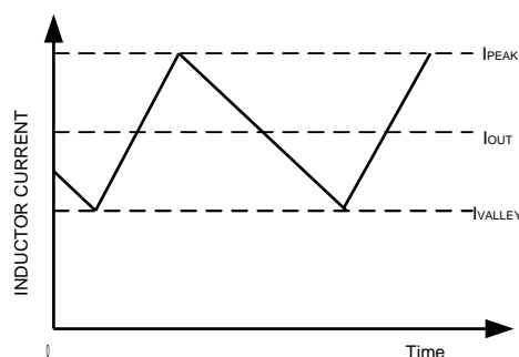
Figure 2. Over-Current Algorithm
