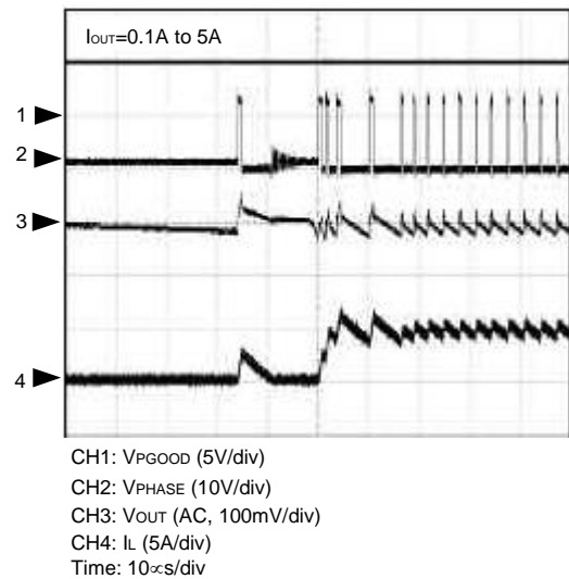
Mode Transient From PFM to PWM
