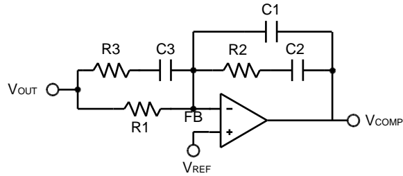
Figure 9. Compensation Network
