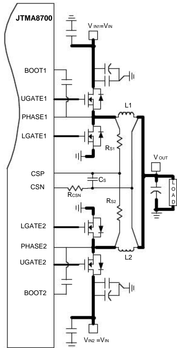
Figure 11. Layout Guidelines
