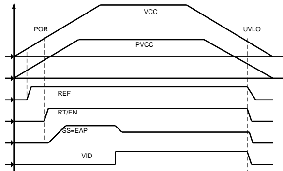
Figure 1. Power on/off sequence
