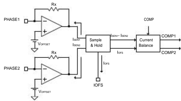
Figure 4. Current balance scheme
