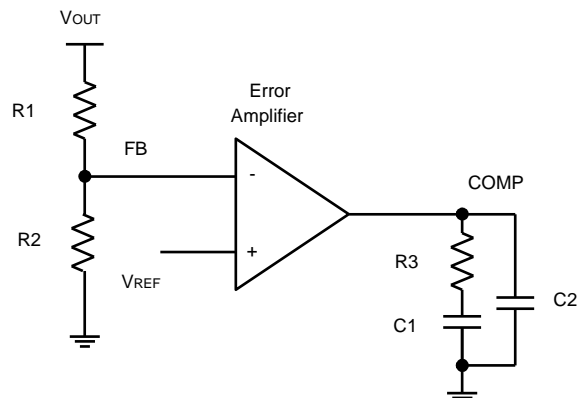
Figure 5. Compensation Network
