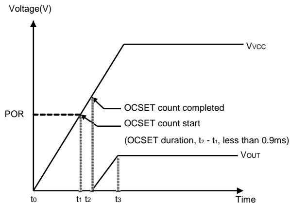
Figure 1. Soft-Start Interval
