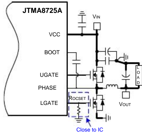
Figure 8. Layout Guidelines
