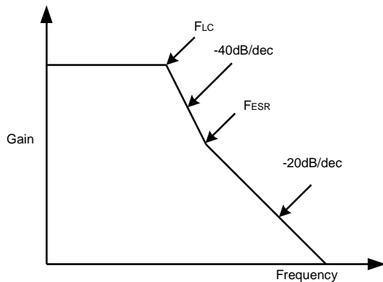
Figure 3. The LC Filter Gain & Frequency
