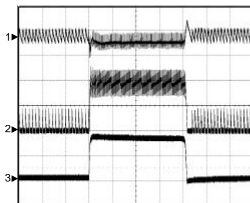
V_{OUT}=1.1V , Load Transient 1A->18A->1A
