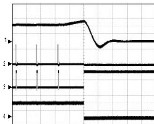
Over-Voltage Protection
