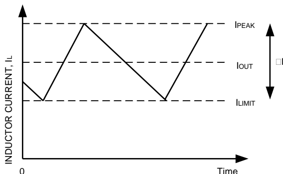
Figure 2. Current-Limit Algorithm
