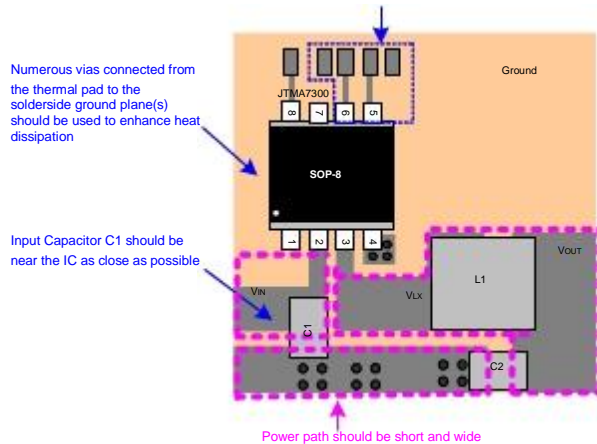
Figure 3. Recommended Layout Diagram
