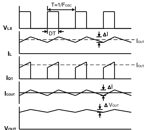
Figure 1. Converter Waveforms
