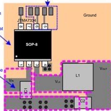
Figure 3. Recommended Layout Diagram
