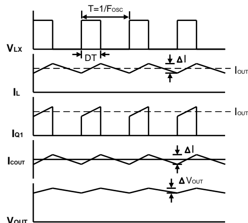
Figure 1. Converter Waveforms
