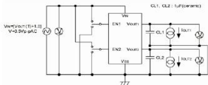
Circuit ⑤
