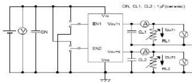
Circuit ①
