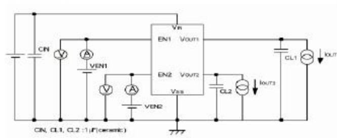
Circuit ④
