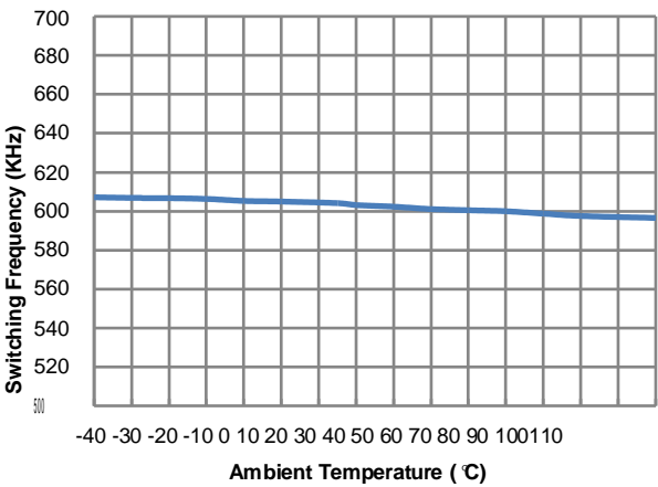
Figure 12. Switching Frequency vs. Temperature
