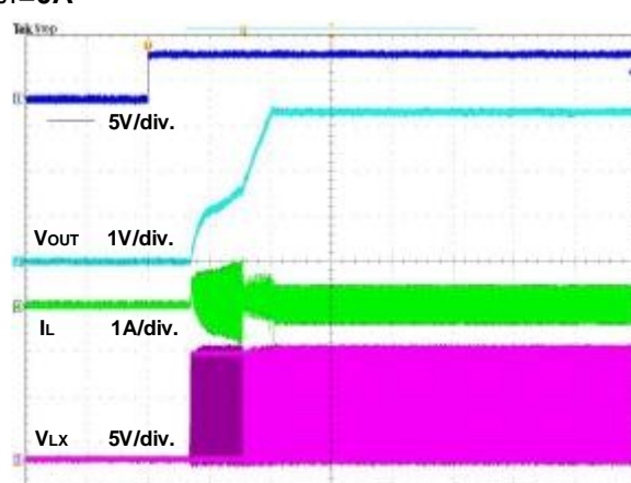
Figure 19. Power On through SH Waveform
