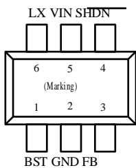
Figure 1. Pin Assignment of JTM2259A
