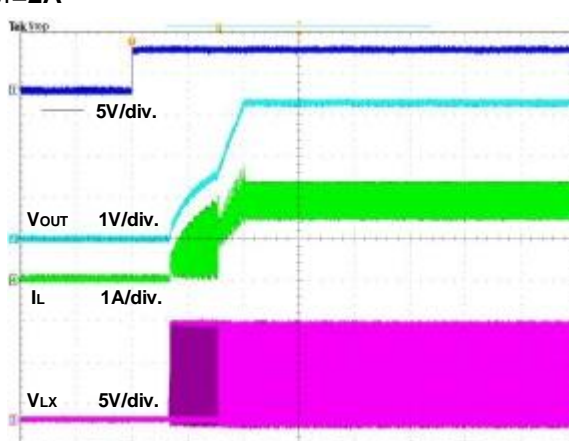
Figure 20. Power On through SH Waveform
