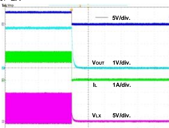
Figure 22. Power Off through SH Waveform
