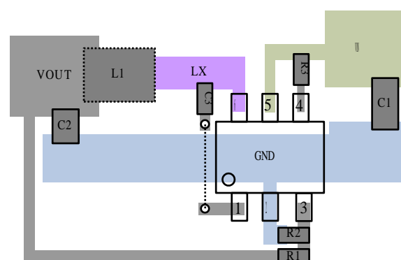
Figure 25. JTM2259A Recommended Layout Diagram
