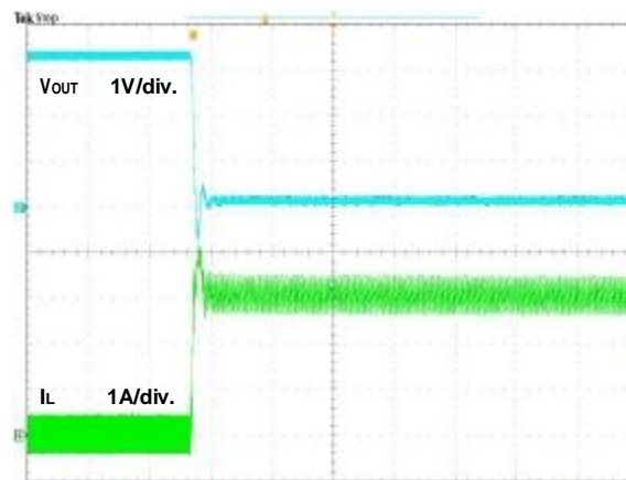
200μs/div. Figure 24. Short Circuit Test
