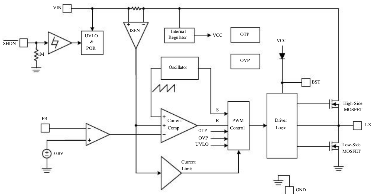
Figure 4. Block Diagram of JTM2259A
