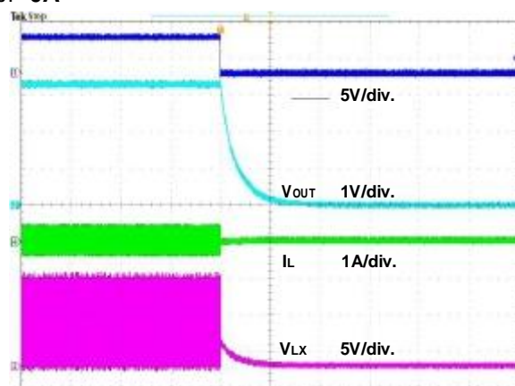
Figure 21. Power Off through SH Waveform
