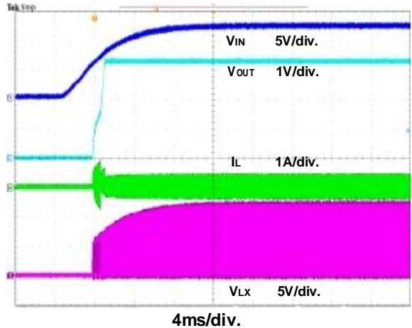
Figure 15. Power On through VIN Waveform
