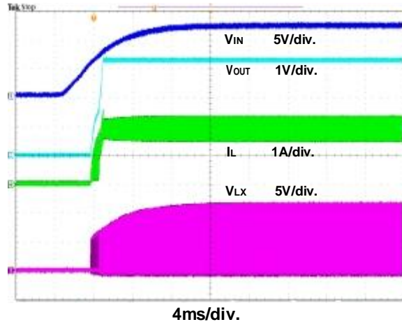
Figure 16. Power On through VIN Waveform
