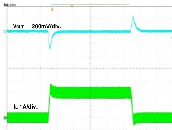
200μs/div. Figure 23. Load Transient Waveform
