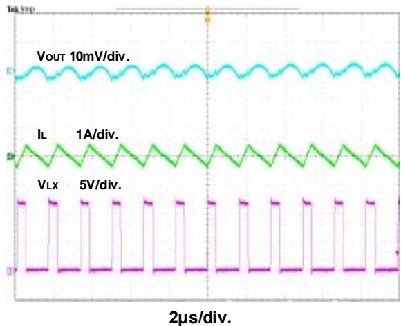
Figure 13. Steady State Waveform
