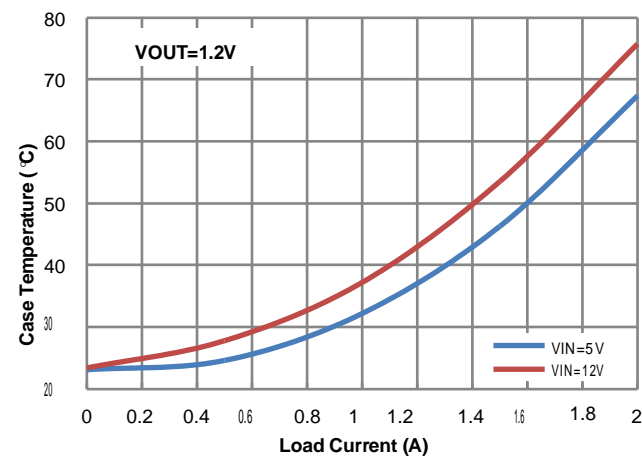
Figure 8. Case Temperature vs. Load Current
