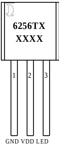
TO-92
