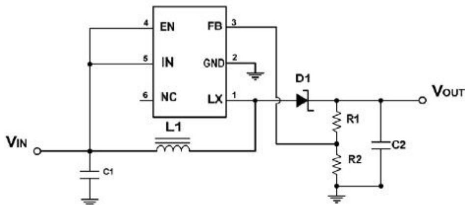
Figure1. Basic Application Circuit
