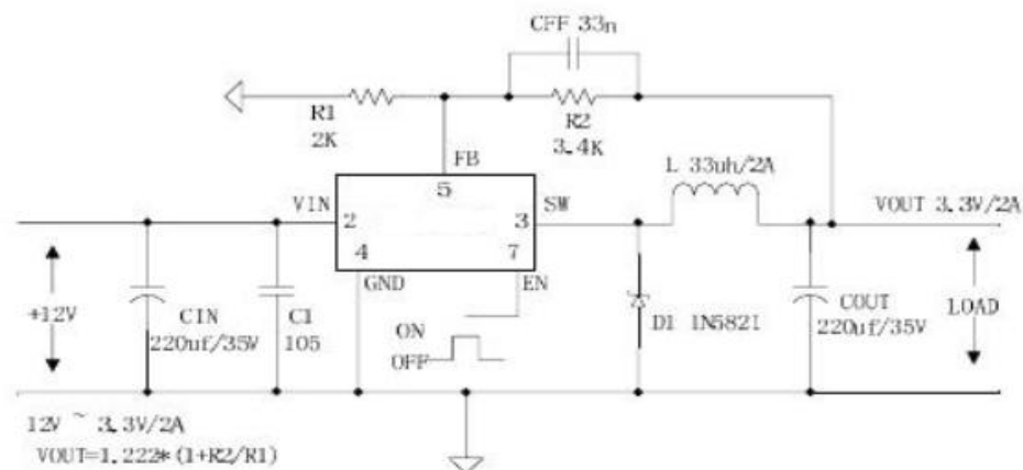
Figure7. JTMX1410 System Parameters Test Circuit (12V ~ 3.3V/2A)
