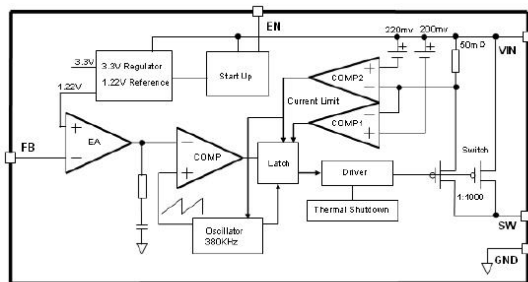
Figure3. Function Block Diagram of JTMX1410
