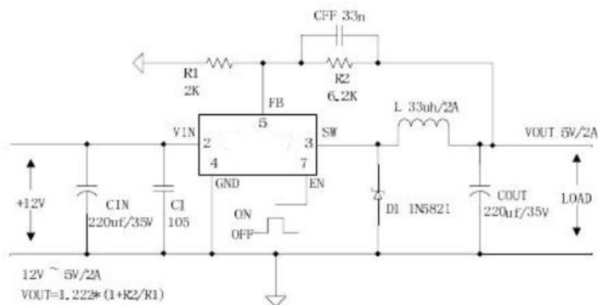
Figure6. JTMX1410 System Parameters Test Circuit (12V ~ 5V/2A)
