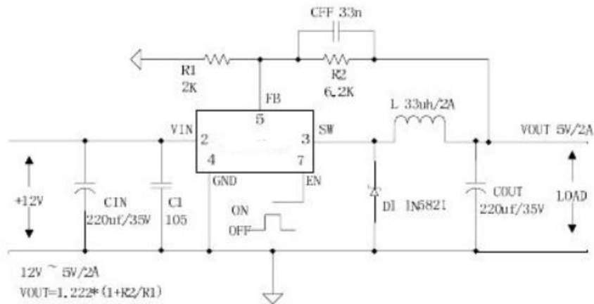
Figure4. JTMX1410 Typical Application Circuit
