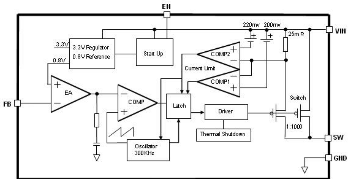
Figure3. Function Block Diagram of JTMX4005
