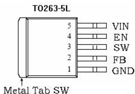
Figure2. Pin Configuration of JTMX4005 (Top View)
