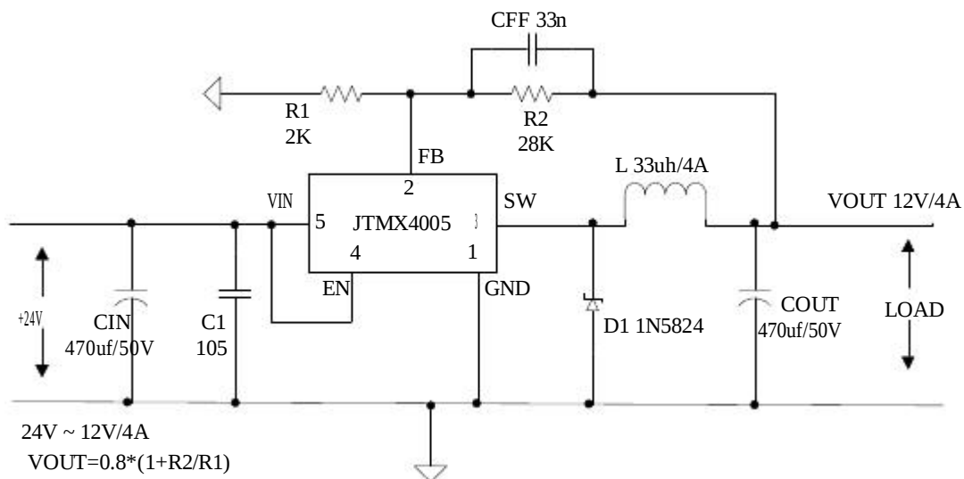
Figure6. JTMX4005 System Parameters Test Circuit (24V ~ 12V/4A)
