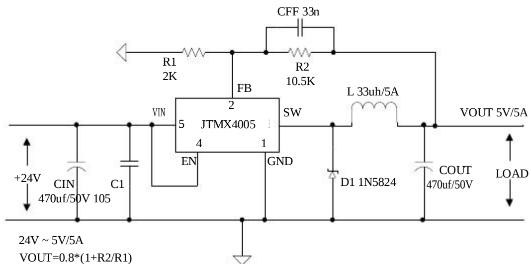
Figure4. JTMX4005 Typical Application Circuit 24V~5V/5A
