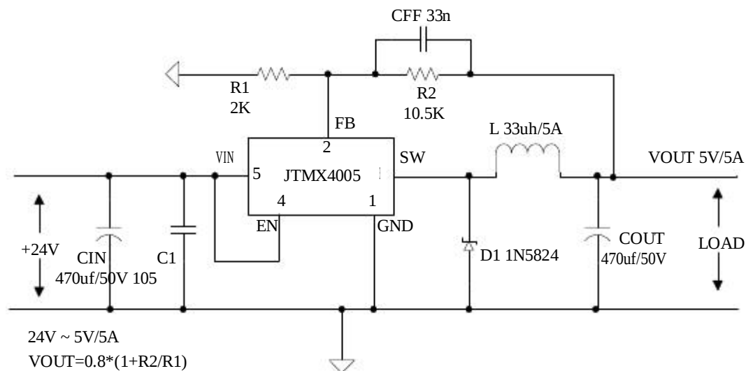
Figure7. JTMX4005 System Parameters Test Circuit (24V ~ 5V/5A)
