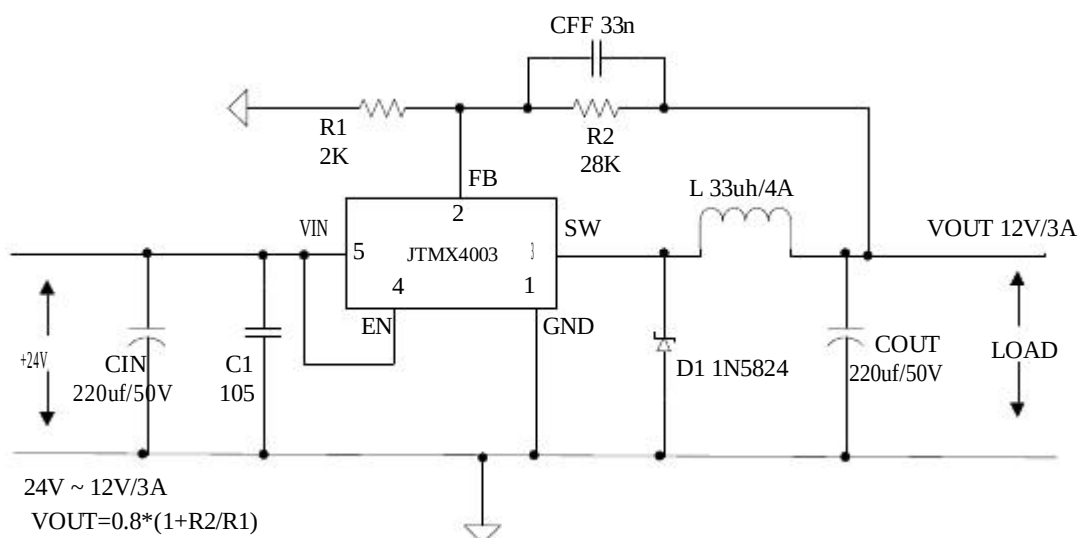
Figure6. JTMX4003 System Parameters Test Circuit (24V ~ 12V/3A)
