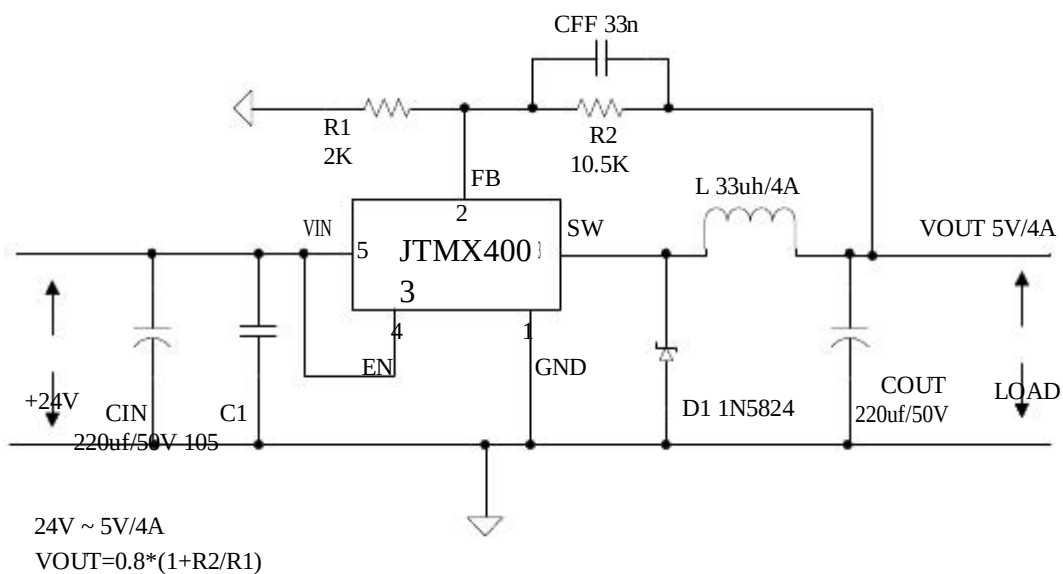
Figure4. JTMX4003 Typical Application Circuit 24V~5V/4A
