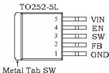
Figure2. Pin Configuration of JTMX4003 (Top View)
