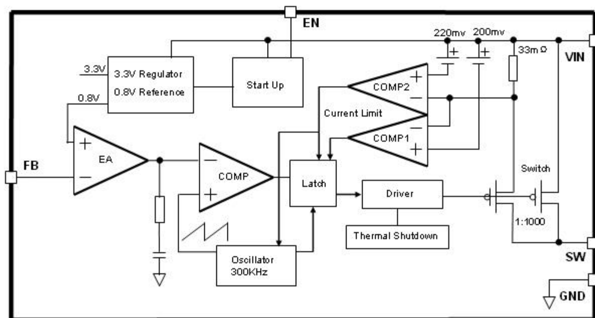
Figure3. Function Block Diagram of JTMX4003
