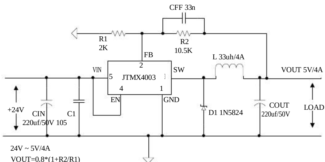
Figure7. JTMX4003 System Parameters Test Circuit (24V ~ 5V/4A)
