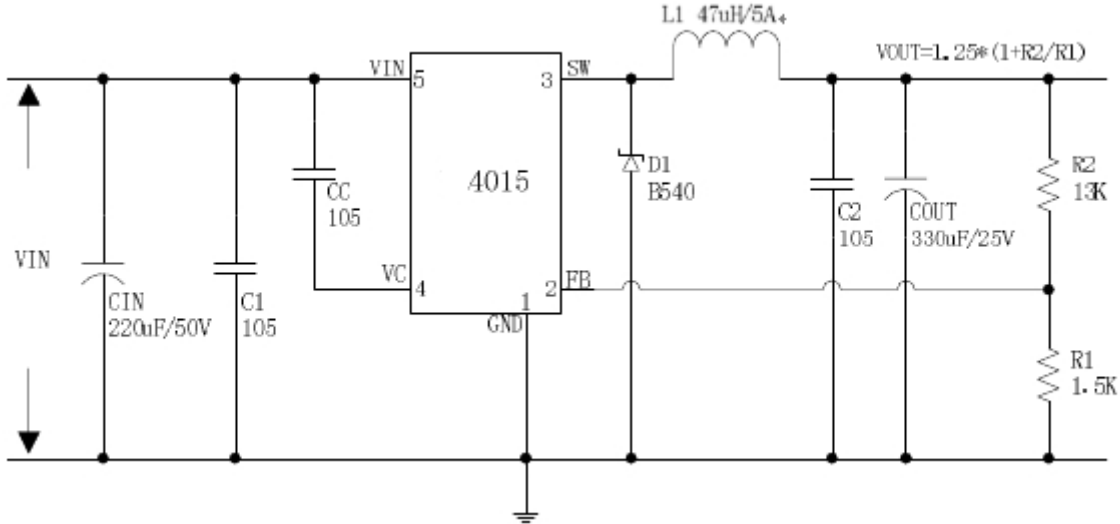
Figure7. JTMX4015 System Parameters Test Circuit (VIN=15V~36V, VOUT=12V/4A)
