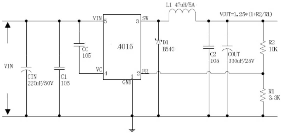
Figure5. JTMX4015 System Parameters Test Circuit (VIN=8V~36V, VOUT=5V/5A)
