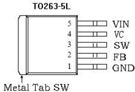
Figure2. Pin Configuration of JTMX4015 (Top View)
