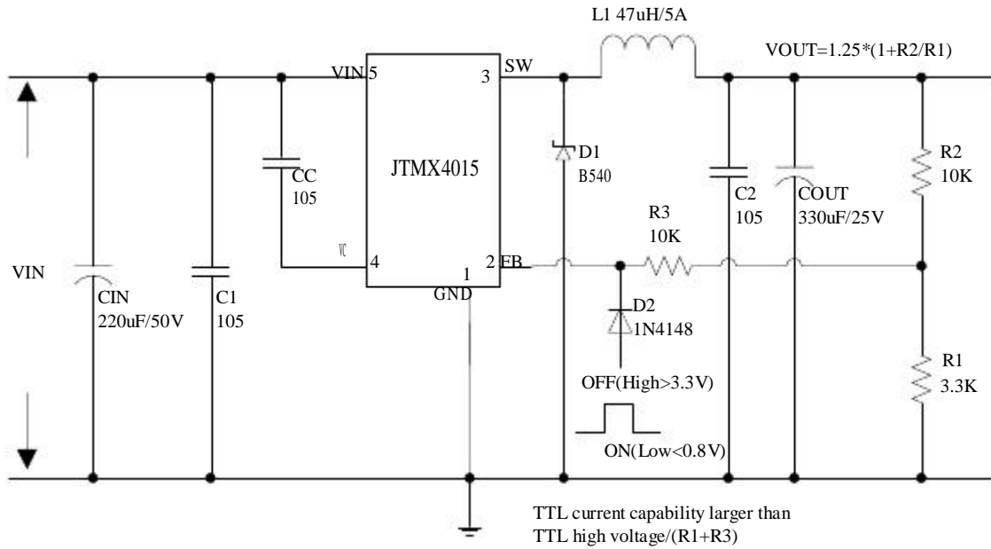
Figure9. JTMX4015 Typical Application Circuit
