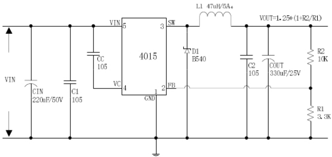
Figure4. JTMX4015 Typical Application Circuit (VIN=8V~36V, VOUT=5V/5A)
