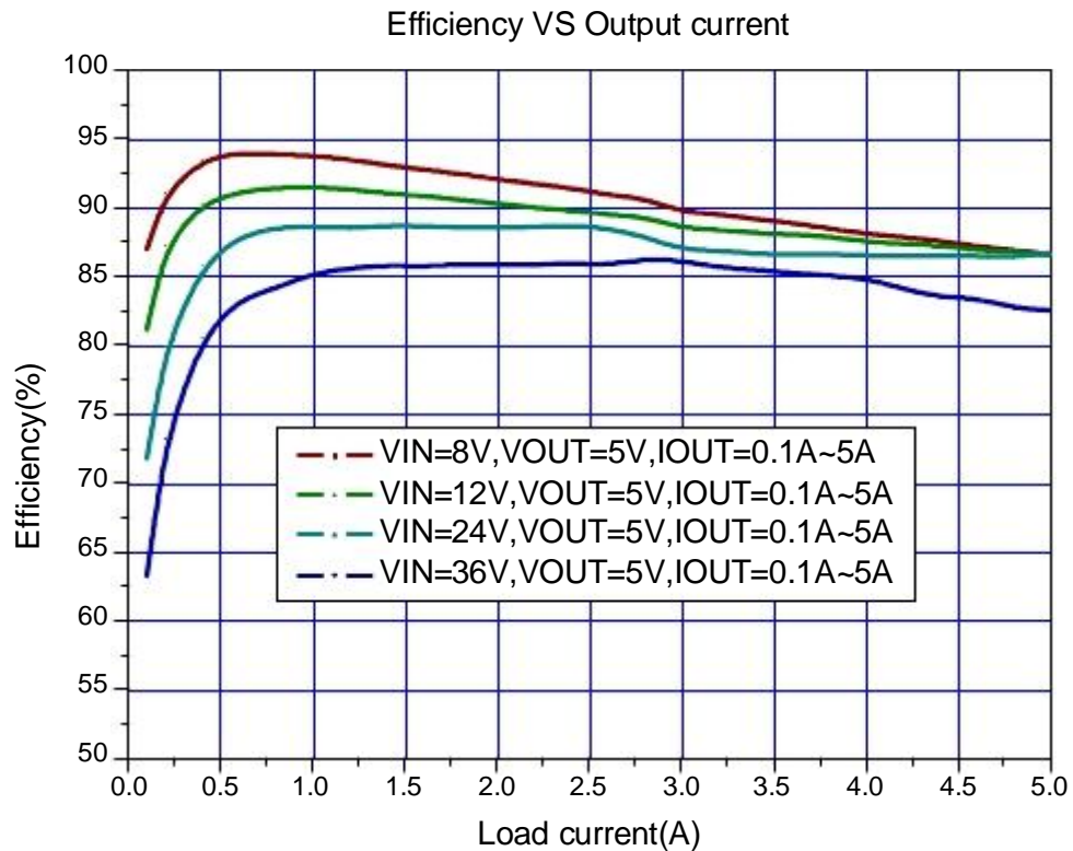
Figure6. JTMX4015 System Efficiency Curve
