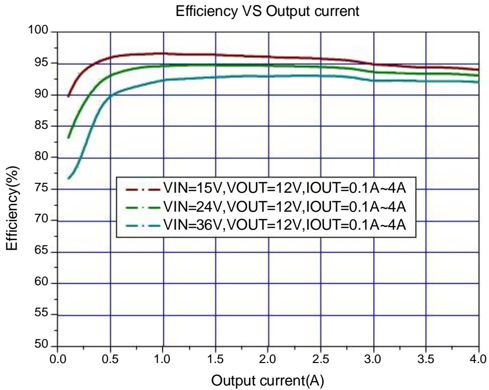
Figure8. JTMX4015 System Efficiency Curve
