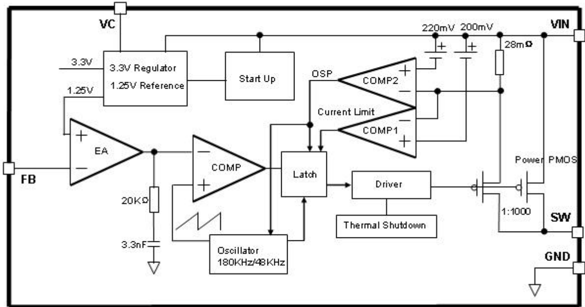
Figure3. Function Block Diagram of JTMX4015
