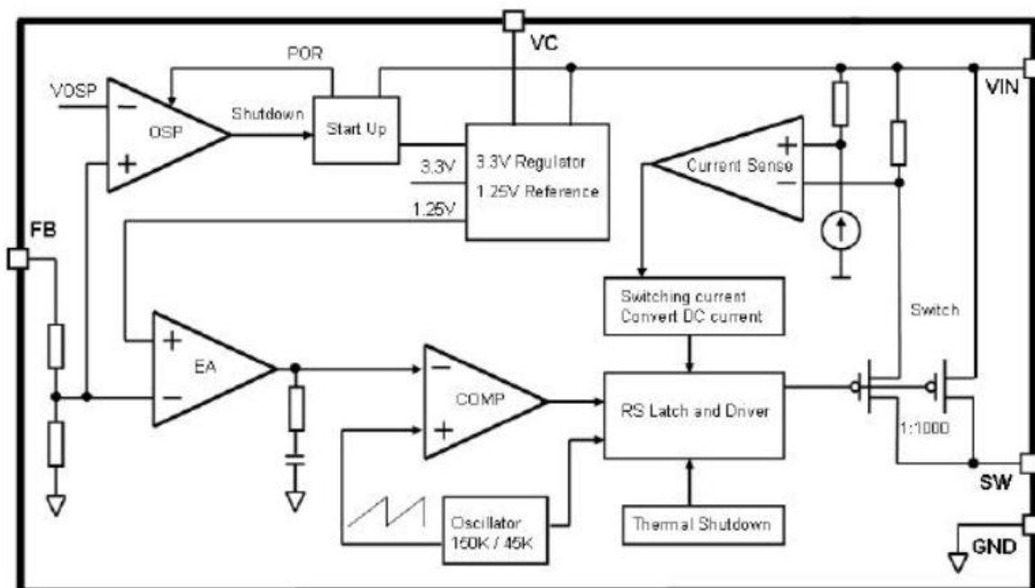
Figure3. Function Block Diagram of JTMX2981
