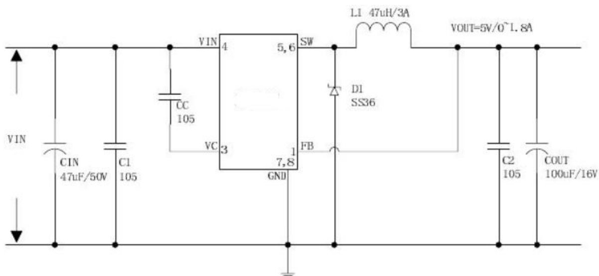
Figure4. JTMX2981 Typical Application Circuit (VIN=8V~45V, VOUT=5V/1.8A)
