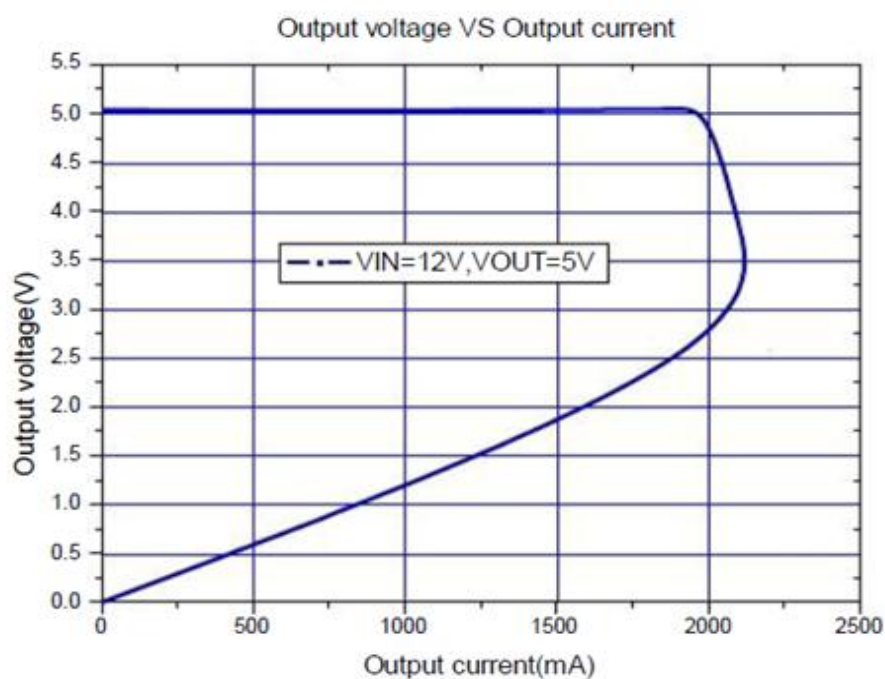
Figure6. JTMX2981 System Output Constant Current Curve
