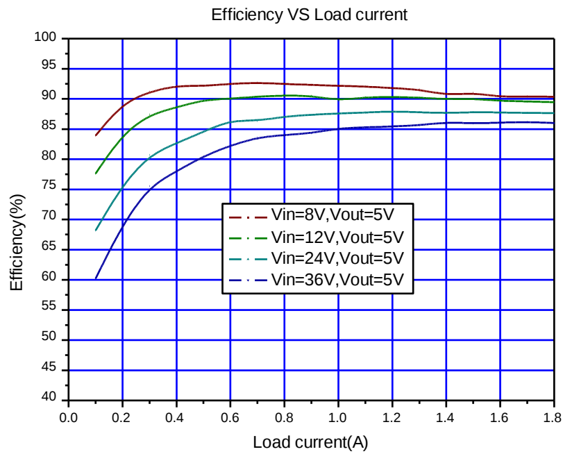
Figure7. JTMX2981 System Efficiency Curve
