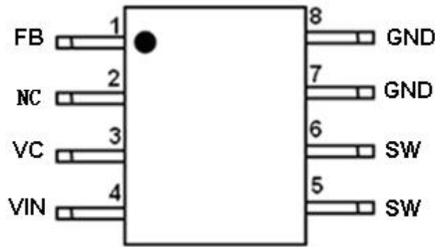
Figure2. Pin Configuration of JTMX2981 (Top View)
