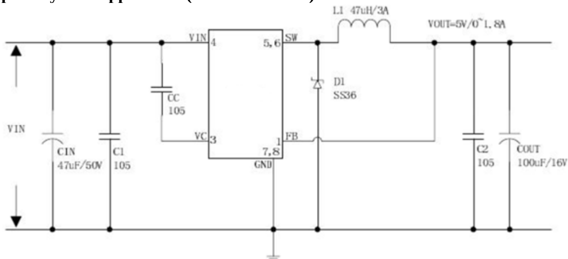
Figure5. JTMX2981System Parameters Test Circuit ( V_{IN}=8V\sim 45V , V_{OUT}=5V/1.8A )
