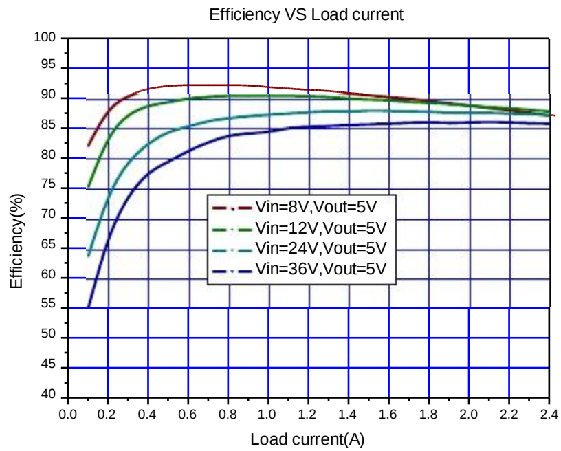
Figure7. JTMX2984 System Efficiency Curve
