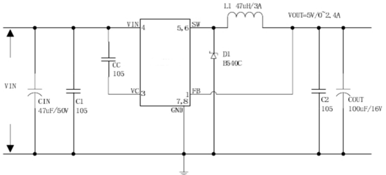
Figure5. JTMX2984 System Parameters Test Circuit (VIN=8V~40V, VOUT=5V/2.4A)
