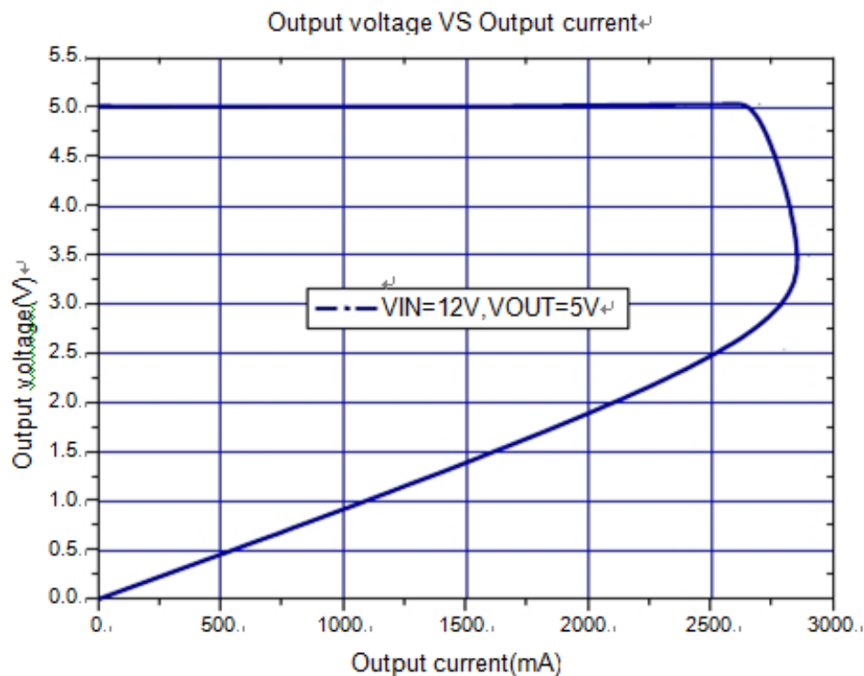
Figure6. JTMX2984 System Output Constant Current Curve
