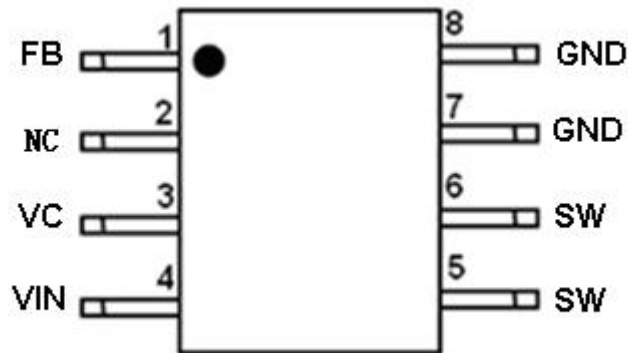
Figure2. Pin Configuration of JTMX2984 (Top View)
