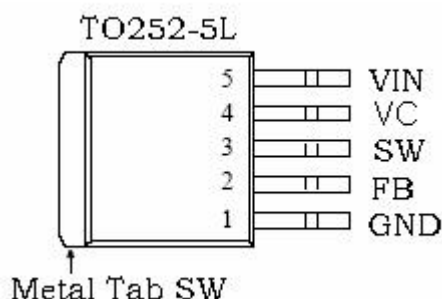
Figure2. Pin Configuration of JTMX2985 (Top View)
