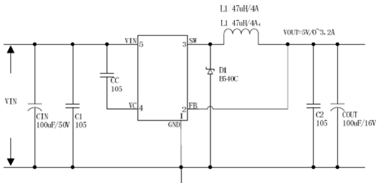
Figure4. JTMX2985 Typical Application Circuit (VIN=8V~40V, VOUT=5V/3.2A)
