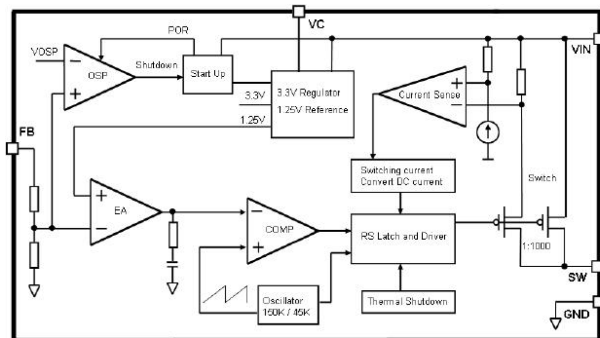
Figure3. Function Block Diagram of JTMX2985
