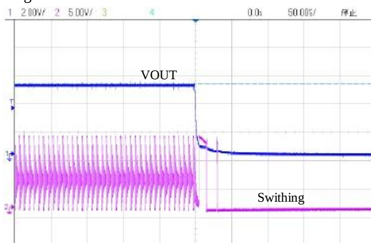
Figure8. The converter will be shutdown when output short happen.
