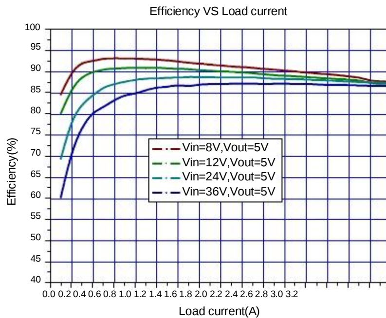
Figure7. JTMX2985 System Efficiency Curve
