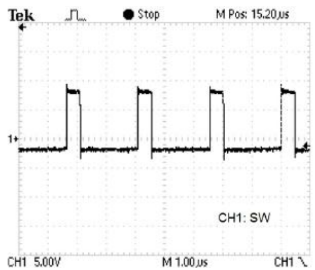
SW ( V_{IN}=9V , V_{OUT}=1.2V , I_{LOAD}=0.5A )
