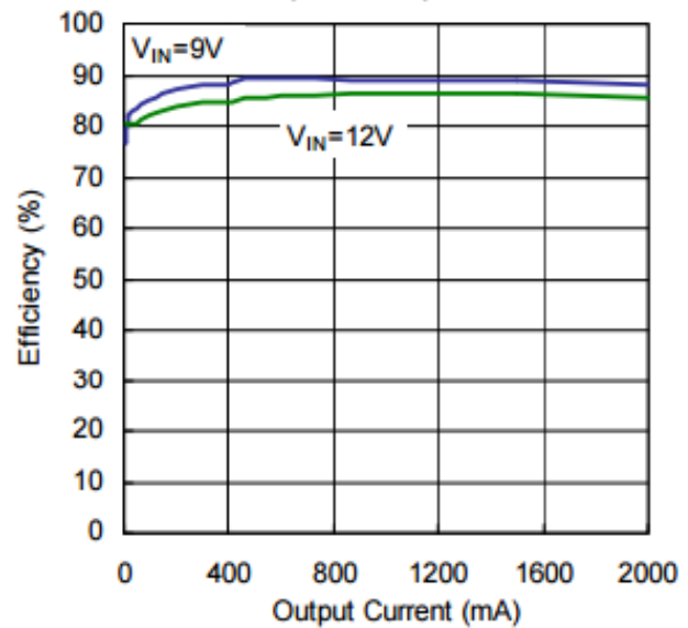
Efficiency vs. Output Current ( V_{OUT}=5\text{V} )
