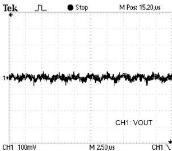
Output Noise ( V_{IN}=9V , V_{OUT}=1.2V , I_{LOAD}=0.5A )
