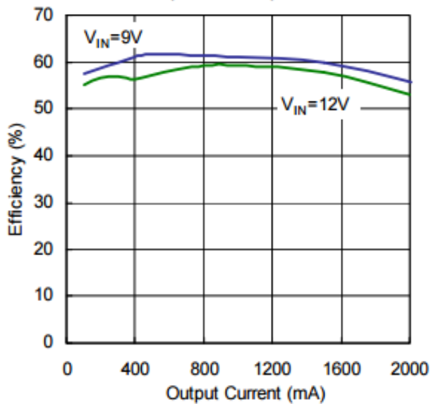
Efficiency vs. Output Current ( V_{OUT}=1.2\text{V} )
