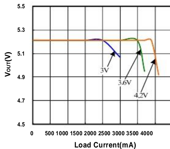
Output Voltage vs Load Current ( V_{out}=5\text{V} )
