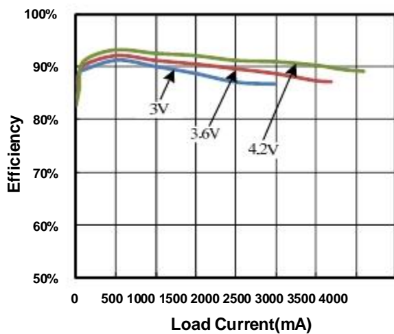
Efficiency vs Load Current ( V_{out}=5\text{V} )
