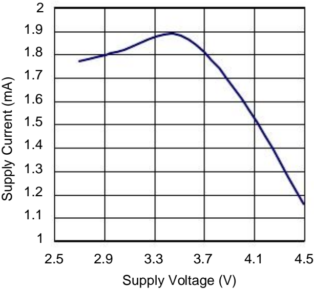
No Load Supply Current vs. Supply Voltage
