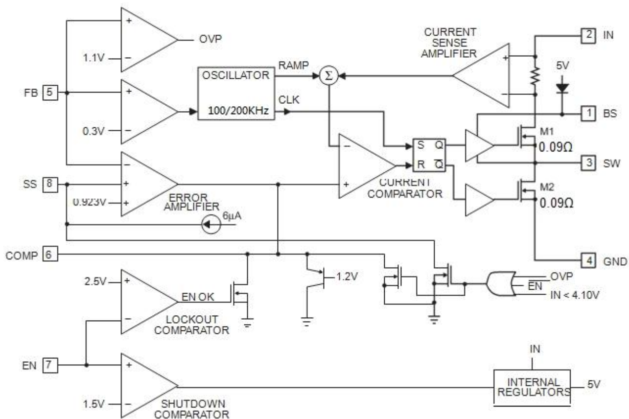
Figure 3 Function Block Diagram of JTMT2778
