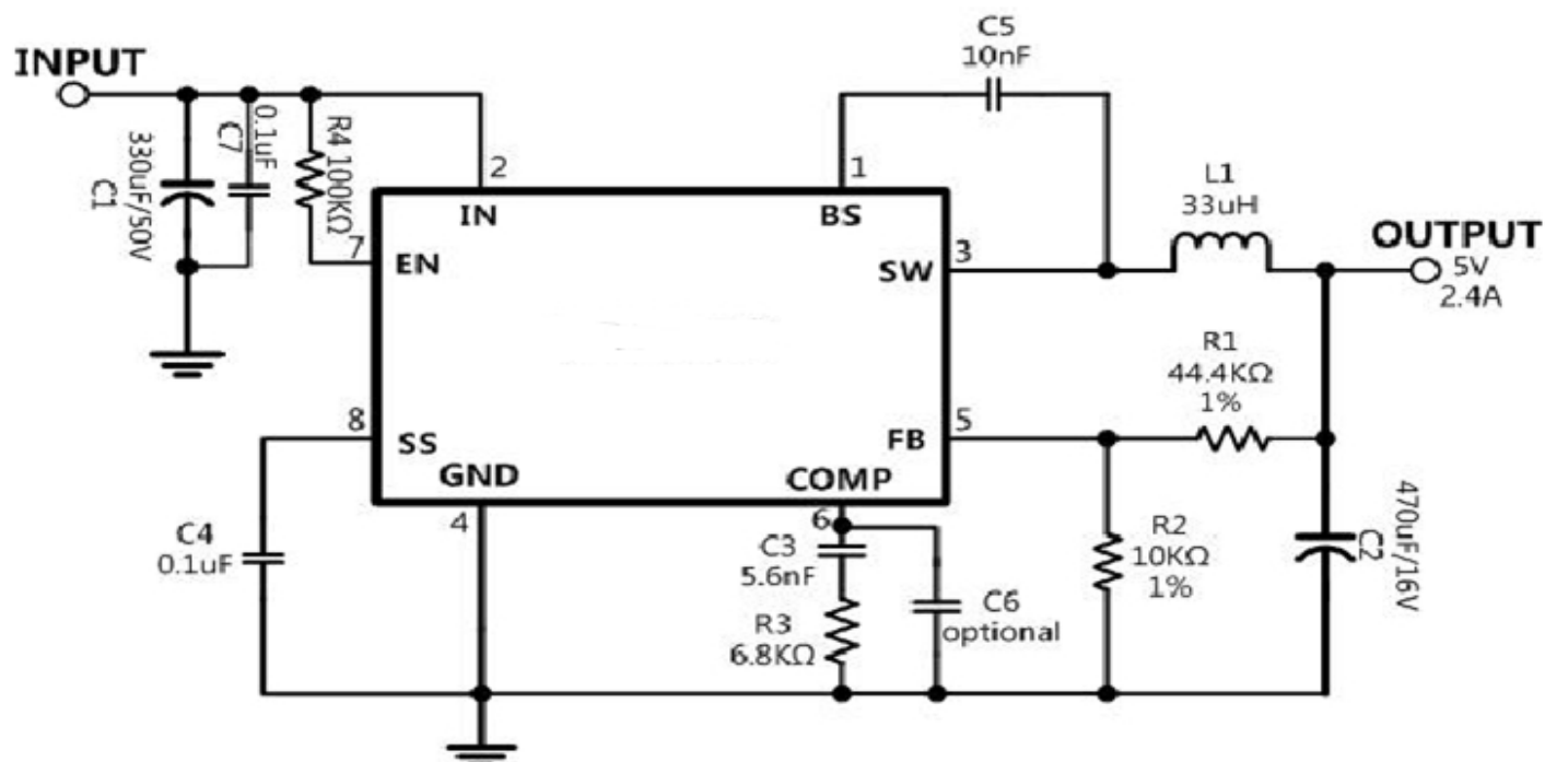
Fig9. JTMT2778 with 5V Output, 470 \mu F/16V Electrolytic Output Capacitor
