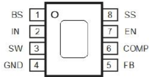
Figure 2 Pin Configuration of JTMT2778(Top View)
