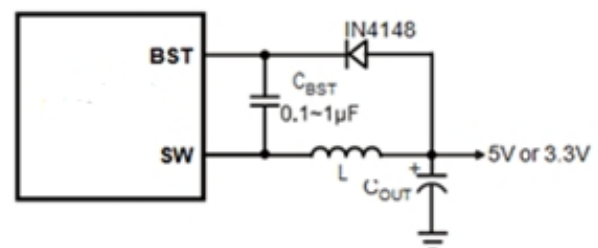
Figure10.Add Optional External Bootstrap Diode to Enhance Efficiency
